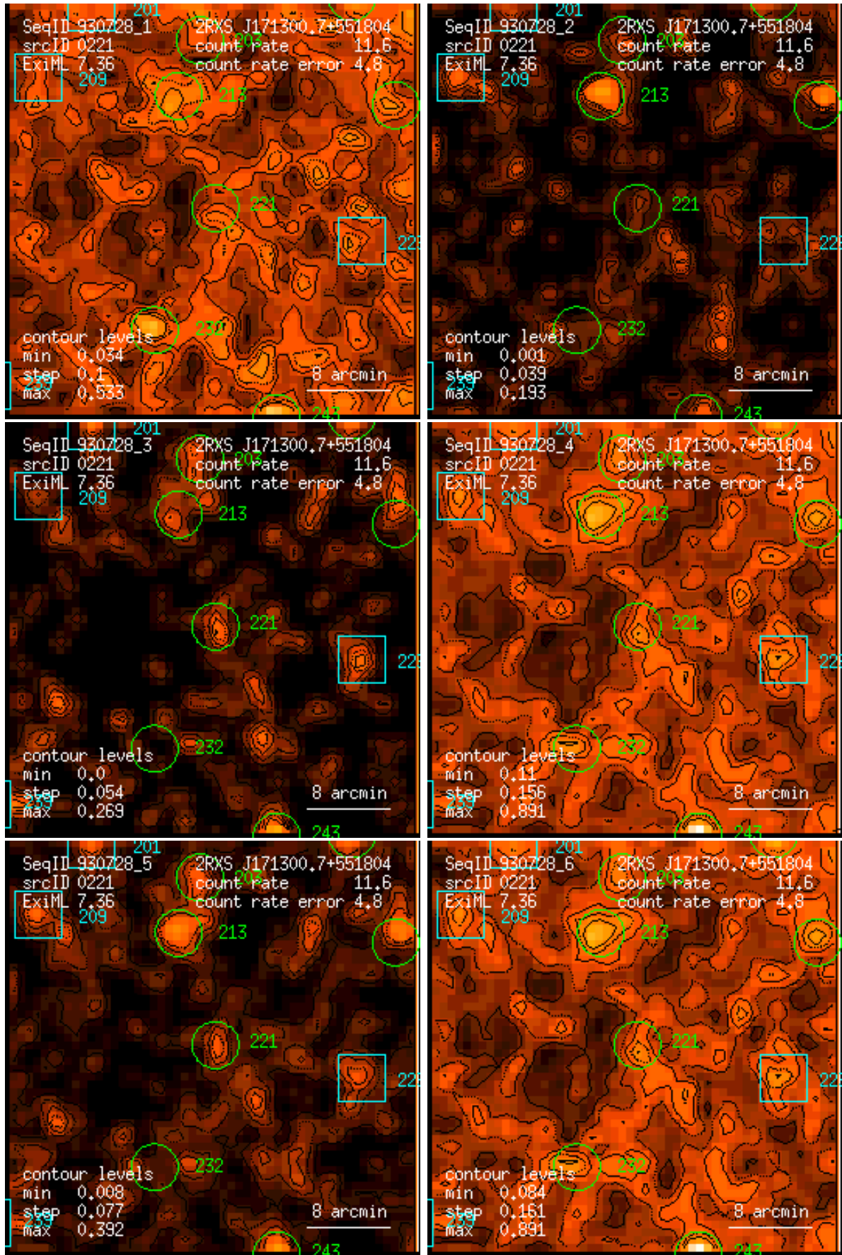
Figure 221: RASS 930728: detection 0221: band rate images, Gaussian filter: (1) PSPC channels 11 – 41, (2) 52 – 90, (3) 91 – 201, (4) 11 – 235, (5) 52 – 201, (6) 11 – 201. Broad band rates in counts/ks. Band rate contour levels in counts/ks/arcmin 2 .
