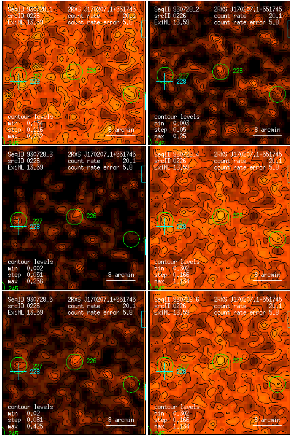
Figure 226: RASS 930728: detection 0226: band rate images, Gaussian filter: (1) PSPC channels 11 – 41, (2) 52 – 90, (3) 91 – 201, (4) 11 – 235, (5) 52 – 201, (6) 11 – 201. Broad band rates in counts/ks. Band rate contour levels in counts/ks/arcmin 2 .
