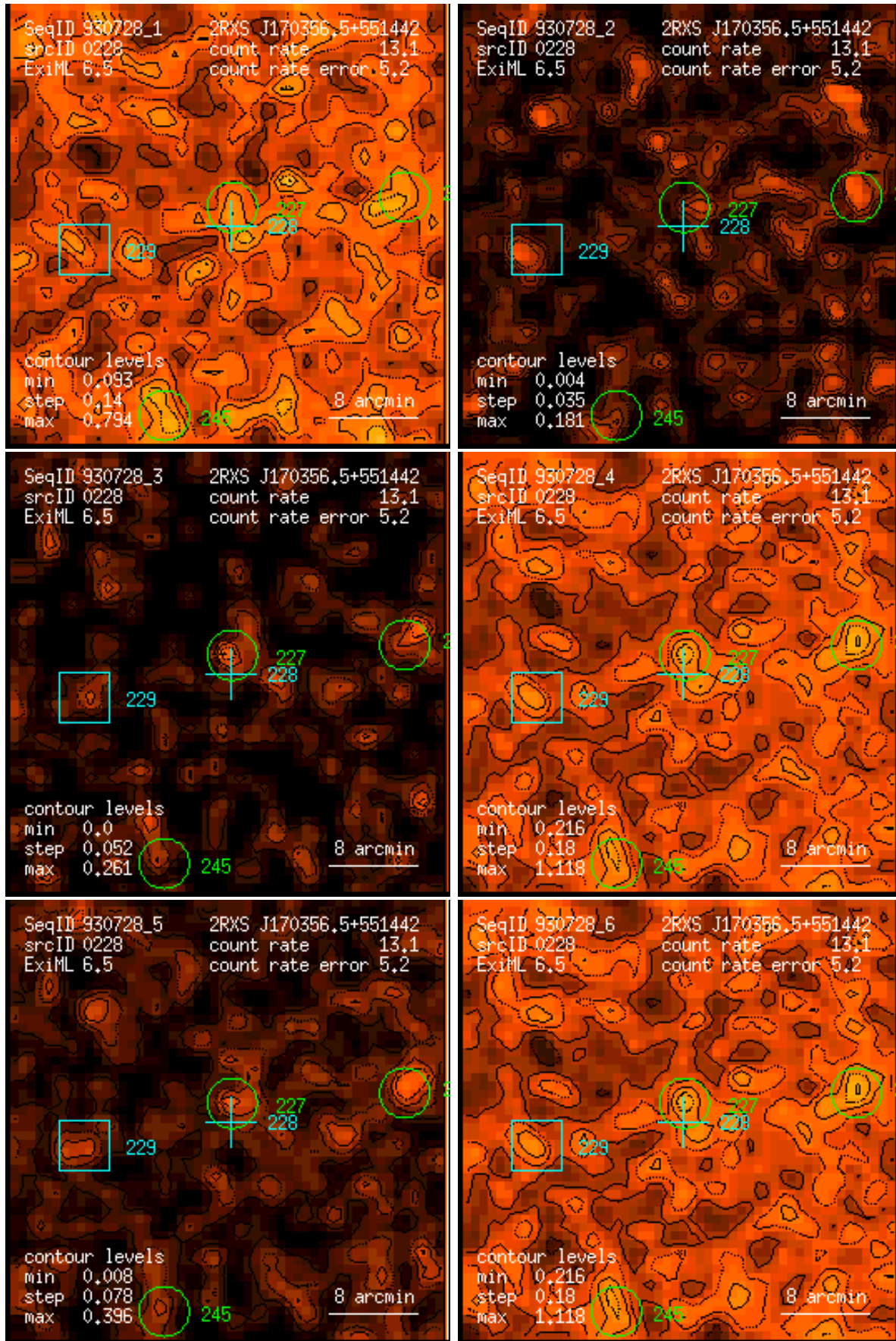
Figure 228: RASS 930728: detection 0228: band rate images, Gaussian filter: (1) PSPC channels 11 – 41, (2) 52 – 90, (3) 91 – 201, (4) 11 – 235, (5) 52 – 201, (6) 11 – 201. Broad band rates in counts/ks. Band rate contour levels in counts/ks/arcmin 2 .
