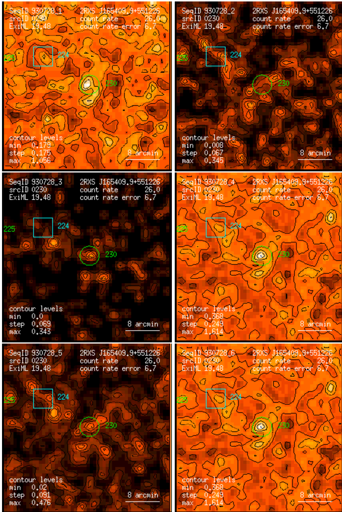
Figure 230: RASS 930728: detection 0230: band rate images, Gaussian filter: (1) PSPC channels 11 – 41, (2) 52 – 90, (3) 91 – 201, (4) 11 – 235, (5) 52 – 201, (6) 11 – 201. Broad band rates in counts/ks. Band rate contour levels in counts/ks/arcmin 2 .
