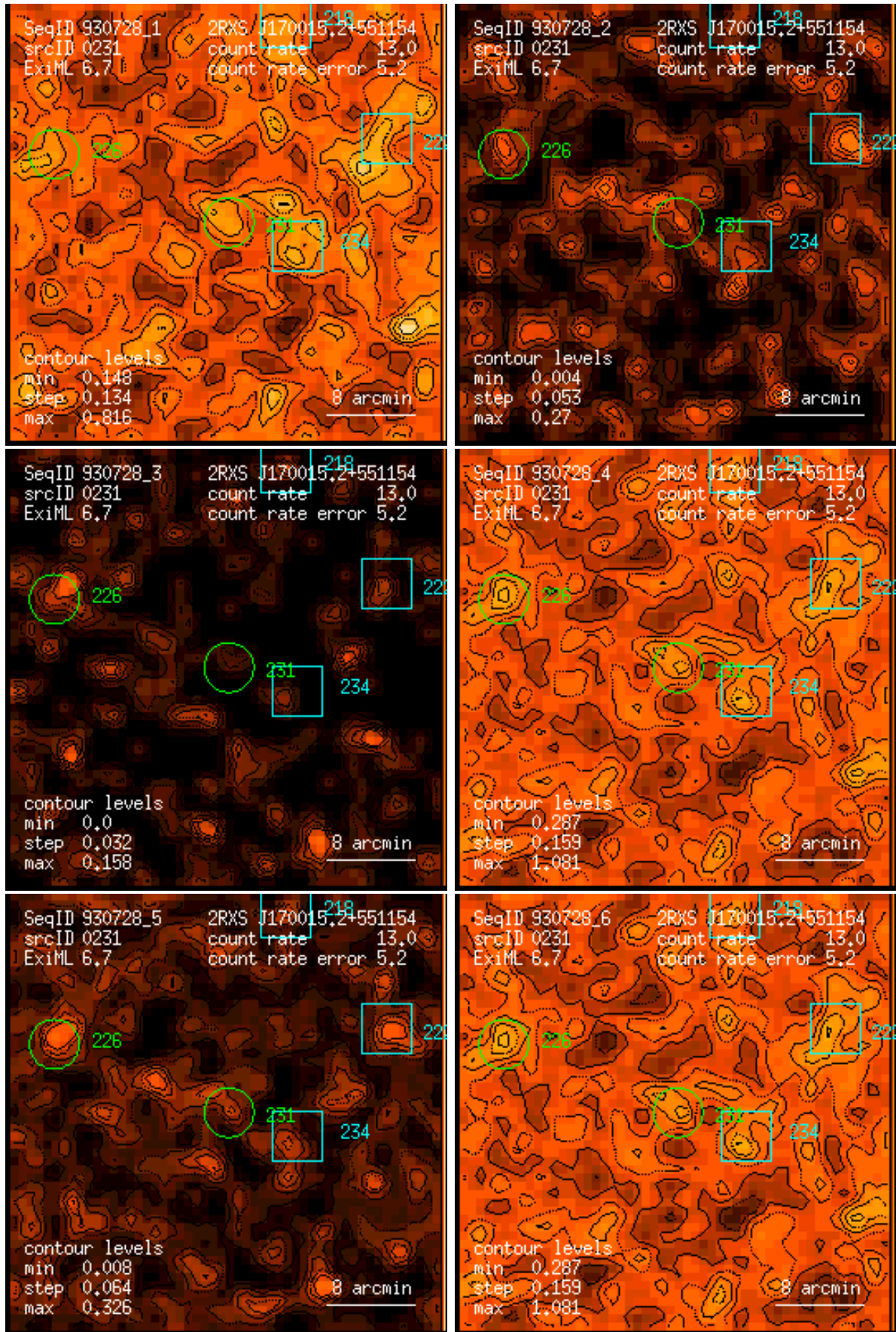
Figure 231: RASS 930728: detection 0231: band rate images, Gaussian filter: (1) PSPC channels 11 – 41, (2) 52 – 90, (3) 91 – 201, (4) 11 – 235, (5) 52 – 201, (6) 11 – 201. Broad band rates in counts/ks. Band rate contour levels in counts/ks/arcmin 2 .
