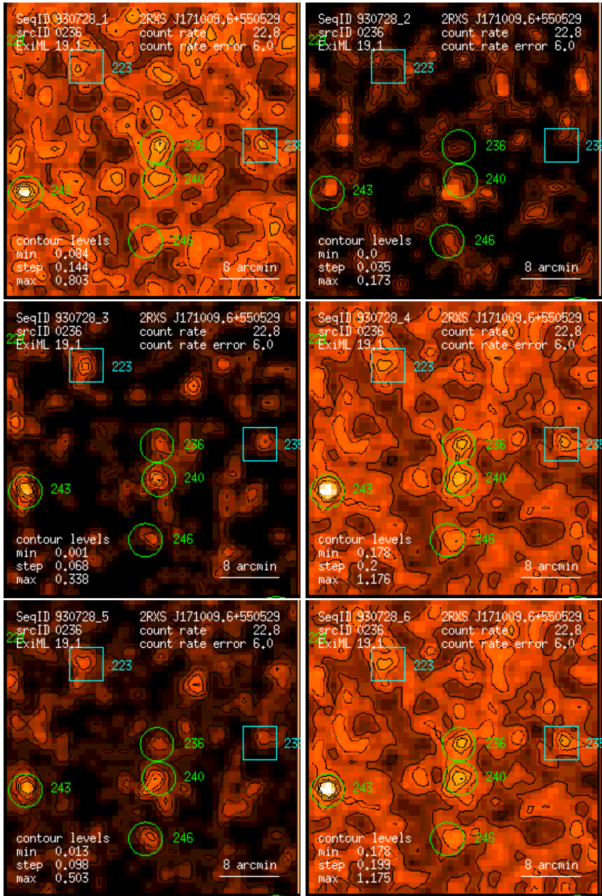
Figure 236: RASS 930728: detection 0236: band rate images, Gaussian filter: (1) PSPC channels 11 – 41, (2) 52 – 90, (3) 91 – 201, (4) 11 – 235, (5) 52 – 201, (6) 11 – 201. Broad band rates in counts/ks. Band rate contour levels in counts/ks/arcmin 2 .
