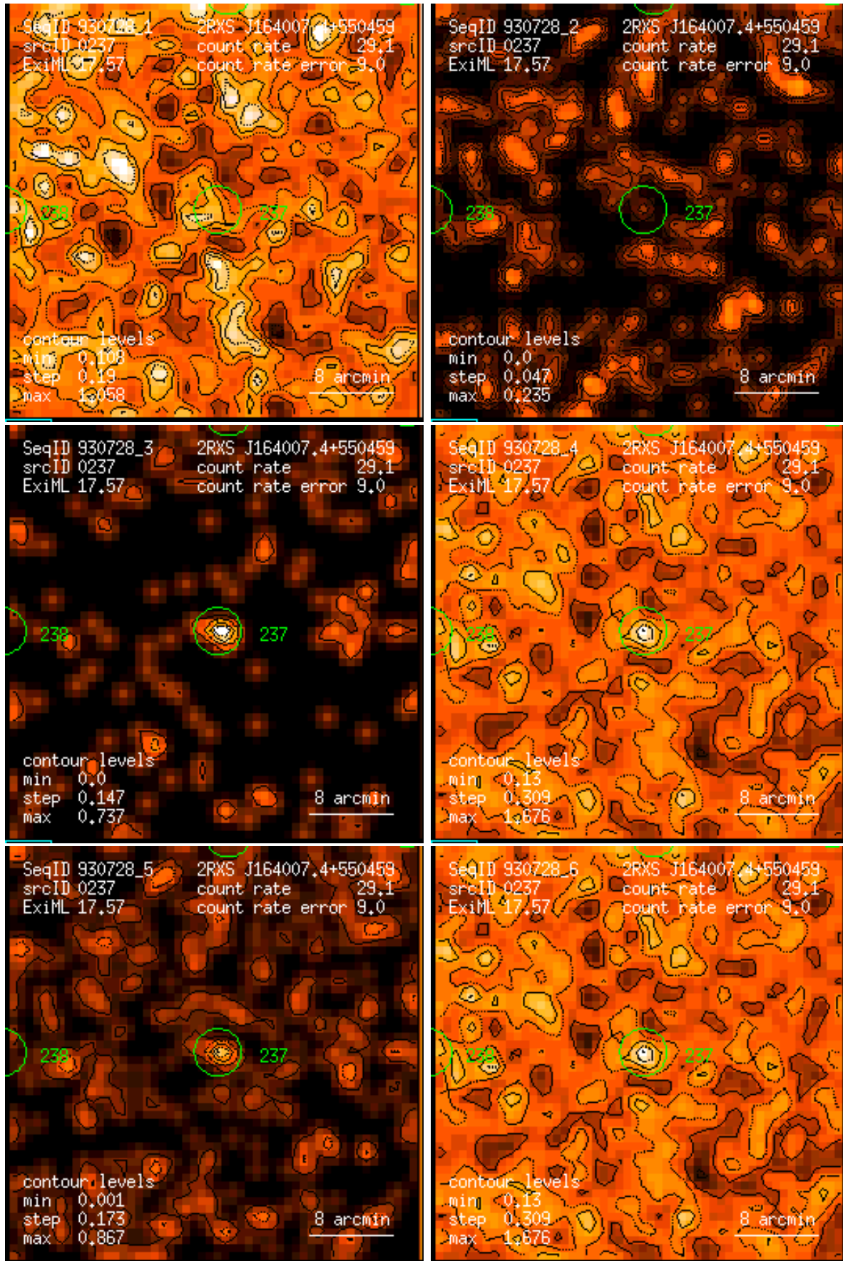
Figure 237: RASS 930728: detection 0237: band rate images, Gaussian filter: (1) PSPC channels 11 – 41, (2) 52 – 90, (3) 91 – 201, (4) 11 – 235, (5) 52 – 201, (6) 11 – 201. Broad band rates in counts/ks. Band rate contour levels in counts/ks/arcmin 2 .
