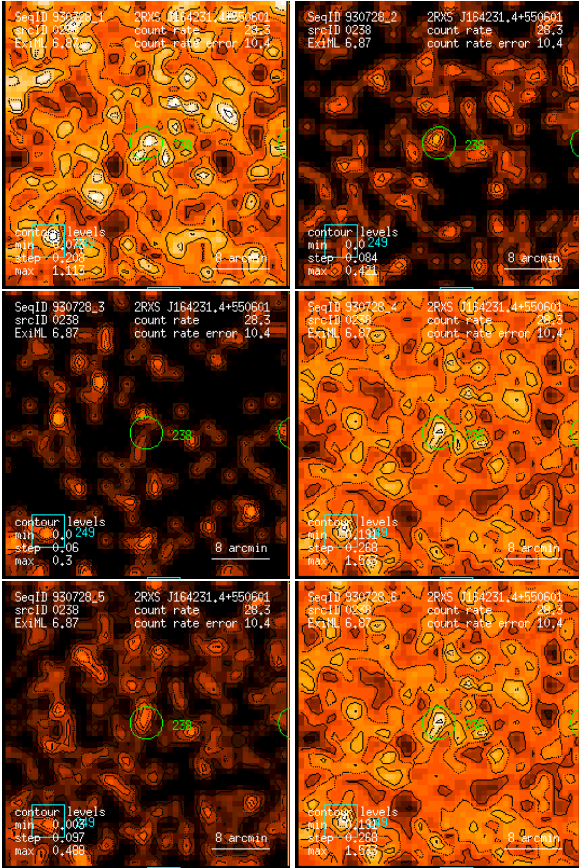
Figure 238: RASS 930728: detection 0238: band rate images, Gaussian filter: (1) PSPC channels 11 – 41, (2) 52 – 90, (3) 91 – 201, (4) 11 – 235, (5) 52 – 201, (6) 11 – 201. Broad band rates in counts/ks. Band rate contour levels in counts/ks/arcmin 2 .
