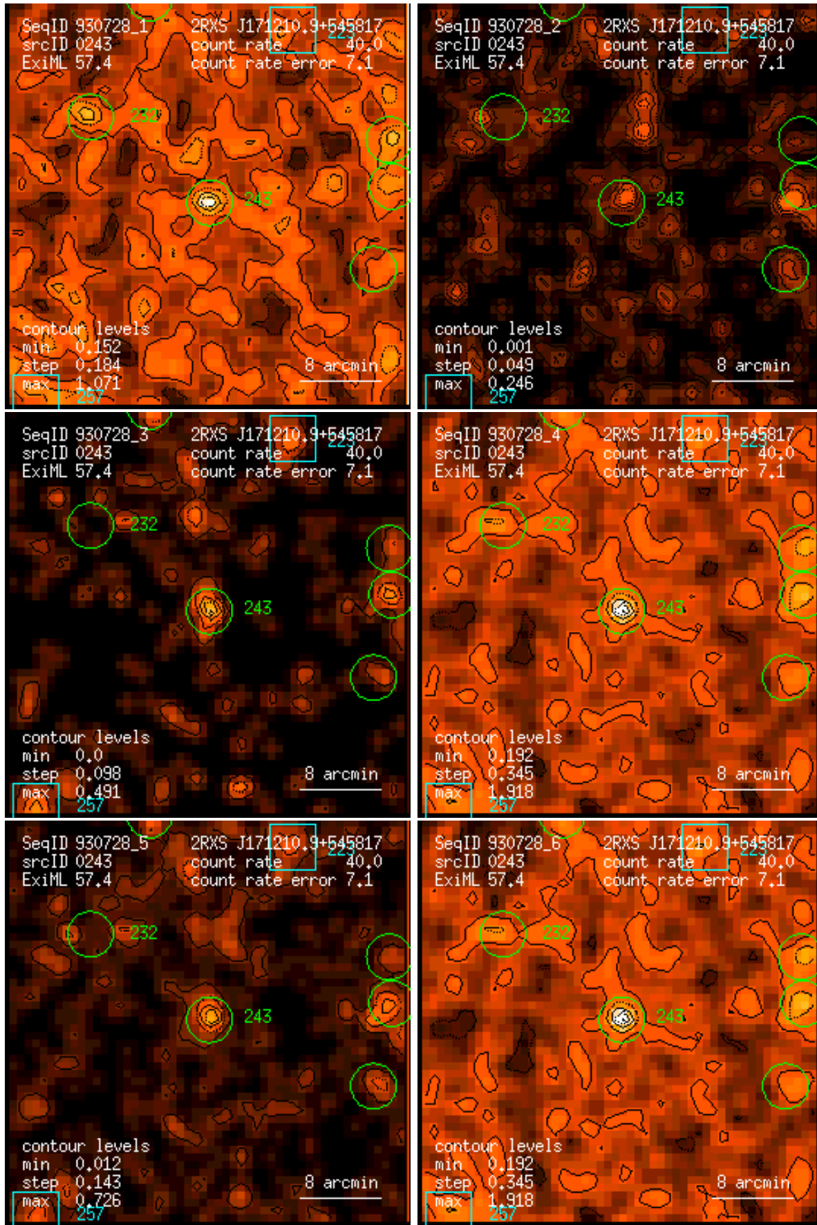
Figure 243: RASS 930728: detection 0243: band rate images, Gaussian filter: (1) PSPC channels 11 – 41, (2) 52 – 90, (3) 91 – 201, (4) 11 – 235, (5) 52 – 201, (6) 11 – 201. Broad band rates in counts/ks. Band rate contour levels in counts/ks/arcmin 2 .
