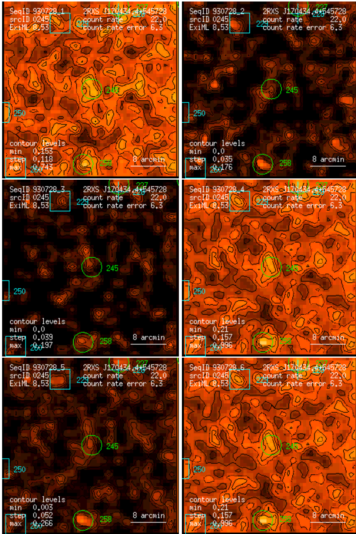
Figure 245: RASS 930728: detection 0245: band rate images, Gaussian filter: (1) PSPC channels 11 – 41, (2) 52 – 90, (3) 91 – 201, (4) 11 – 235, (5) 52 – 201, (6) 11 – 201. Broad band rates in counts/ks. Band rate contour levels in counts/ks/arcmin 2 .
