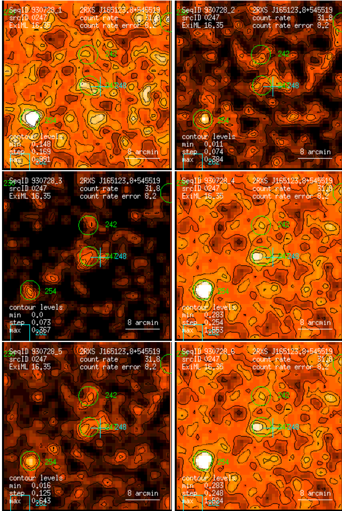
Figure 247: RASS 930728: detection 0247: band rate images, Gaussian filter: (1) PSPC channels 11 – 41, (2) 52 – 90, (3) 91 – 201, (4) 11 – 235, (5) 52 – 201, (6) 11 – 201. Broad band rates in counts/ks. Band rate contour levels in counts/ks/arcmin 2 .
