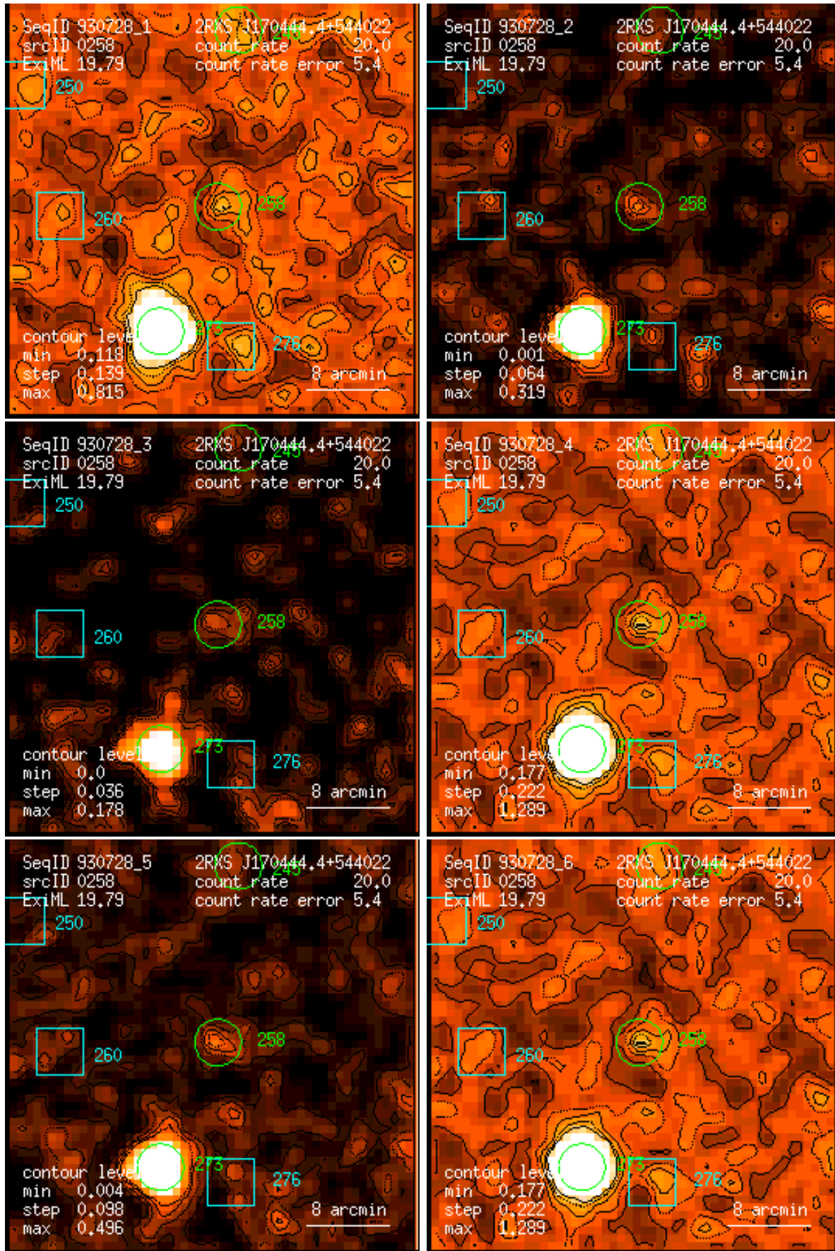
Figure 258: RASS 930728: detection 0258: band rate images, Gaussian filter: (1) PSPC channels 11 – 41, (2) 52 – 90, (3) 91 – 201, (4) 11 – 235, (5) 52 – 201, (6) 11 – 201. Broad band rates in counts/ks. Band rate contour levels in counts/ks/arcmin 2 .
