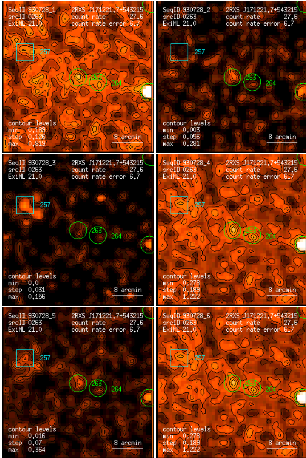
Figure 263: RASS 930728: detection 0263: band rate images, Gaussian filter: (1) PSPC channels 11 – 41, (2) 52 – 90, (3) 91 – 201, (4) 11 – 235, (5) 52 – 201, (6) 11 – 201. Broad band rates in counts/ks. Band rate contour levels in counts/ks/arcmin 2 .
