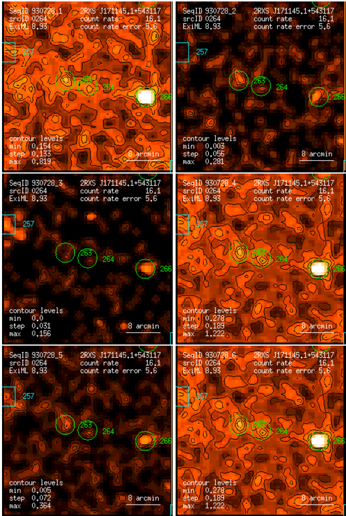
Figure 264: RASS 930728: detection 0264: band rate images, Gaussian filter: (1) PSPC channels 11 – 41, (2) 52 – 90, (3) 91 – 201, (4) 11 – 235, (5) 52 – 201, (6) 11 – 201. Broad band rates in counts/ks. Band rate contour levels in counts/ks/arcmin 2 .
