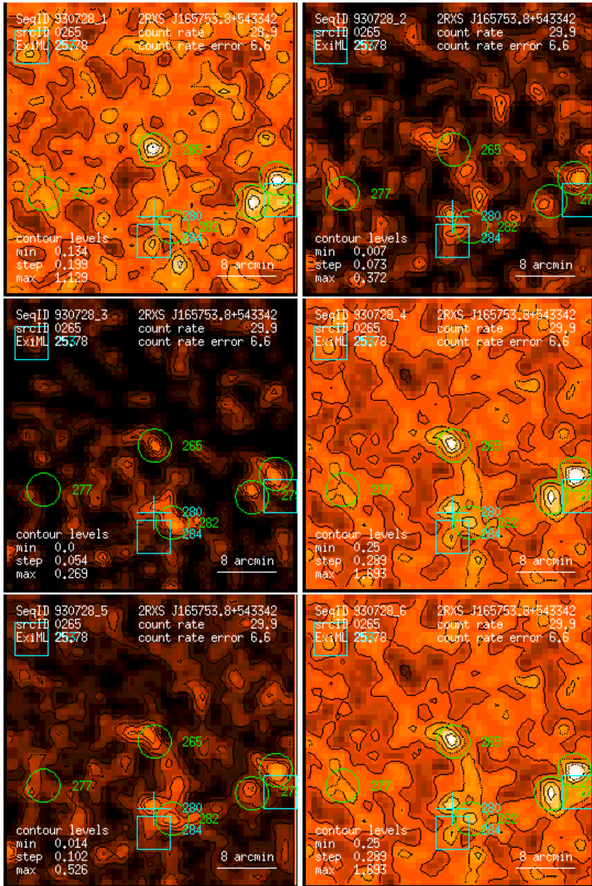
Figure 265: RASS 930728: detection 0265: band rate images, Gaussian filter: (1) PSPC channels 11 – 41, (2) 52 – 90, (3) 91 – 201, (4) 11 – 235, (5) 52 – 201, (6) 11 – 201. Broad band rates in counts/ks. Band rate contour levels in counts/ks/arcmin 2 .
