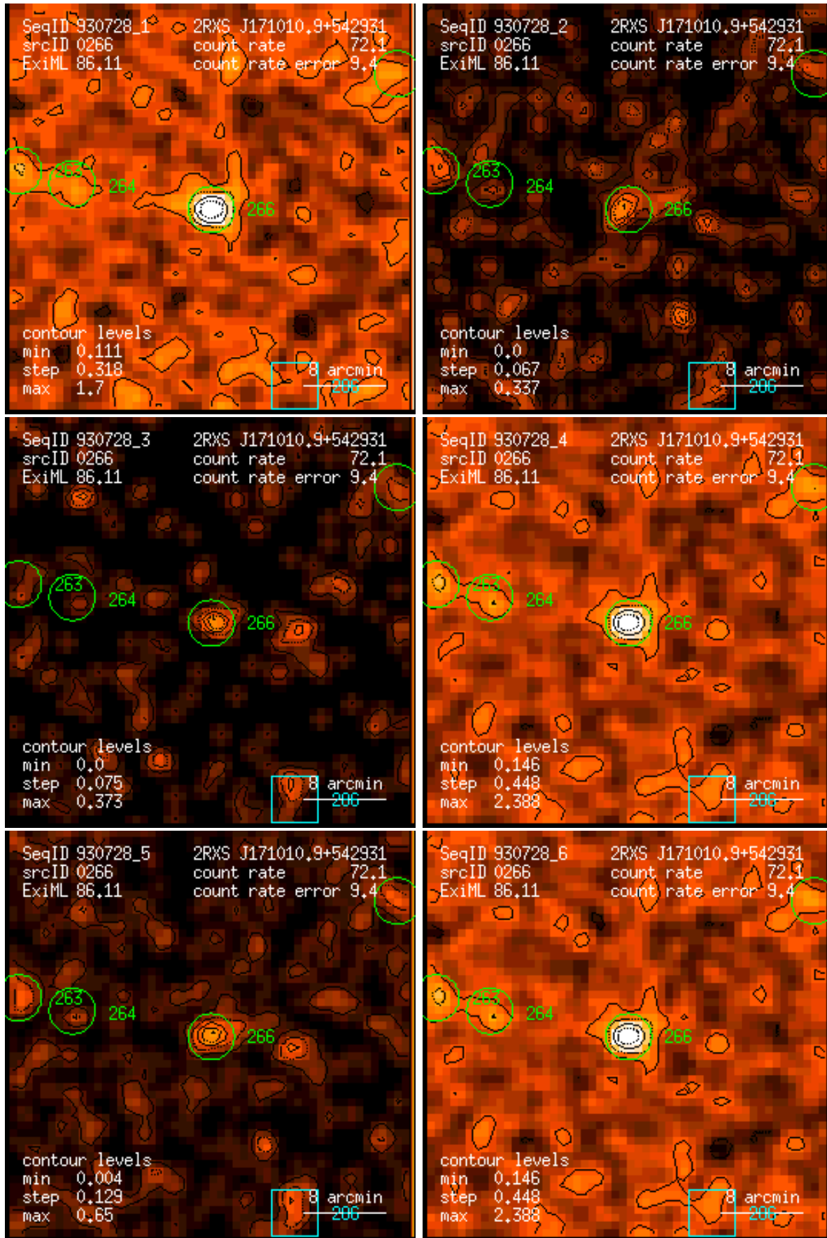
Figure 266: RASS 930728: detection 0266: band rate images, Gaussian filter: (1) PSPC channels 11 – 41, (2) 52 – 90, (3) 91 – 201, (4) 11 – 235, (5) 52 – 201, (6) 11 – 201. Broad band rates in counts/ks. Band rate contour levels in counts/ks/arcmin 2 .
