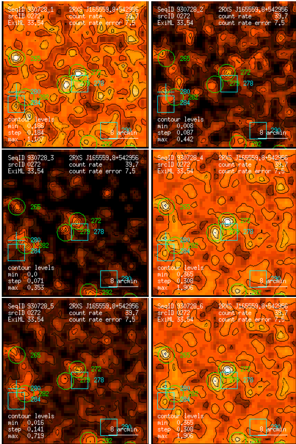
Figure 272: RASS 930728: detection 0272: band rate images, Gaussian filter: (1) PSPC channels 11 – 41, (2) 52 – 90, (3) 91 – 201, (4) 11 – 235, (5) 52 – 201, (6) 11 – 201. Broad band rates in counts/ks. Band rate contour levels in counts/ks/arcmin 2 .
