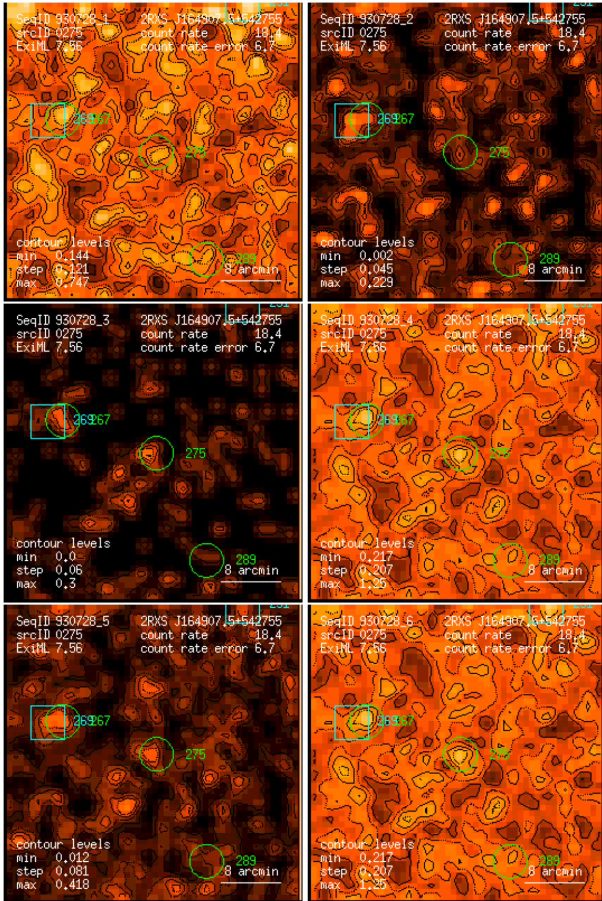
Figure 275: RASS 930728: detection 0275: band rate images, Gaussian filter: (1) PSPC channels 11 – 41, (2) 52 – 90, (3) 91 – 201, (4) 11 – 235, (5) 52 – 201, (6) 11 – 201. Broad band rates in counts/ks. Band rate contour levels in counts/ks/arcmin 2 .
