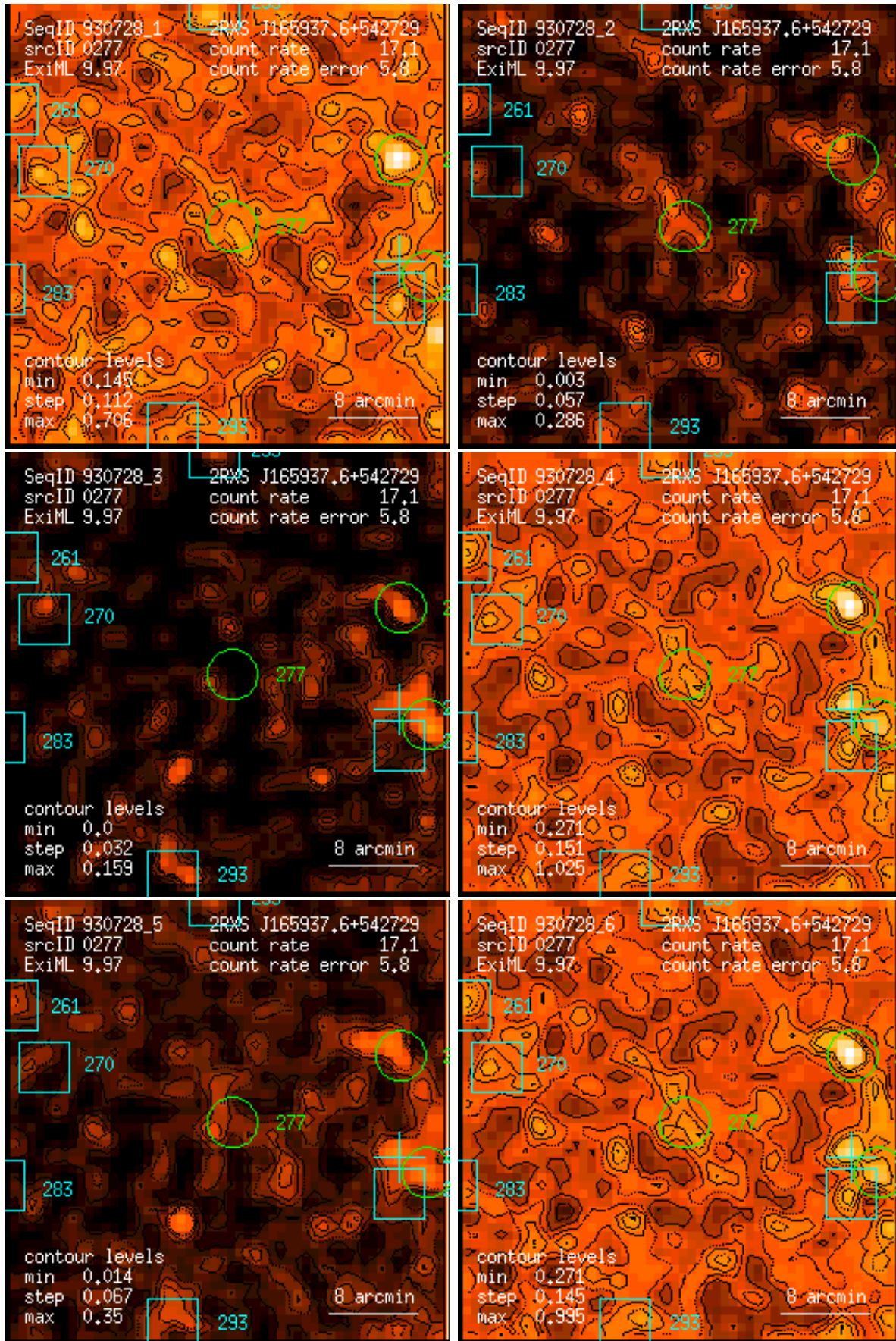
Figure 277: RASS 930728: detection 0277: band rate images, Gaussian filter: (1) PSPC channels 11 – 41, (2) 52 – 90, (3) 91 – 201, (4) 11 – 235, (5) 52 – 201, (6) 11 – 201. Broad band rates in counts/ks. Band rate contour levels in counts/ks/arcmin 2 .
