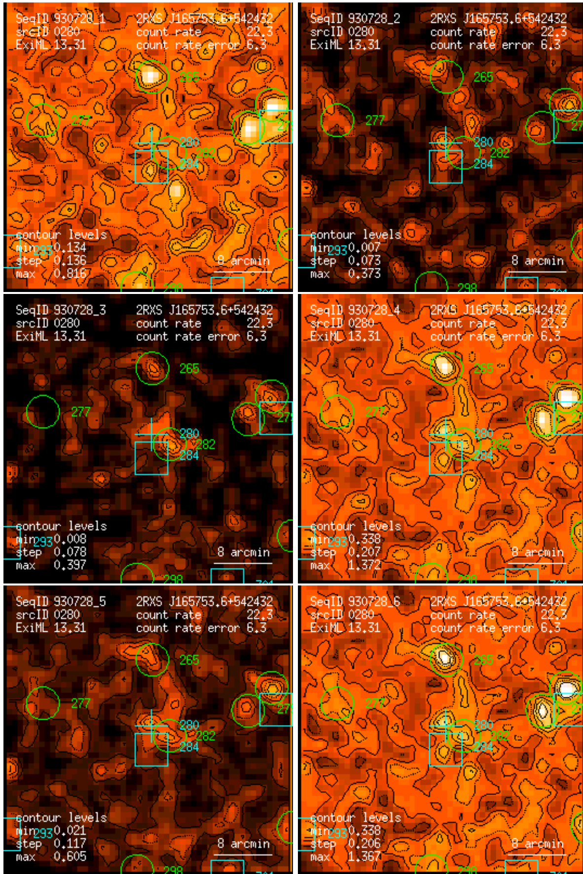
Figure 280: RASS 930728: detection 0280: band rate images, Gaussian filter: (1) PSPC channels 11 – 41, (2) 52 – 90, (3) 91 – 201, (4) 11 – 235, (5) 52 – 201, (6) 11 – 201. Broad band rates in counts/ks. Band rate contour levels in counts/ks/arcmin 2 .
