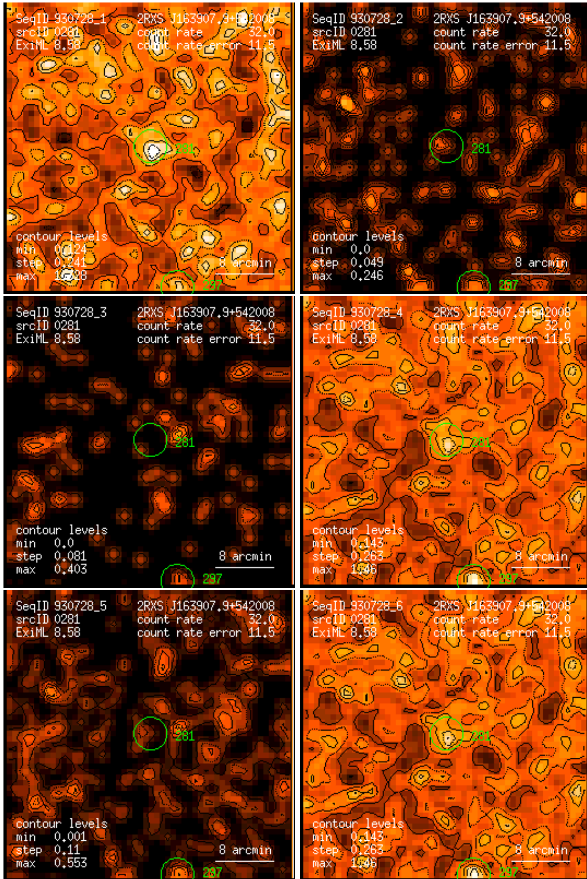
Figure 281: RASS 930728: detection 0281: band rate images, Gaussian filter: (1) PSPC channels 11 – 41, (2) 52 – 90, (3) 91 – 201, (4) 11 – 235, (5) 52 – 201, (6) 11 – 201. Broad band rates in counts/ks. Band rate contour levels in counts/ks/arcmin 2 .
