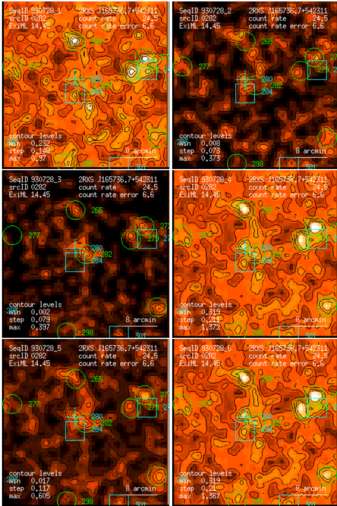
Figure 282: RASS 930728: detection 0282: band rate images, Gaussian filter: (1) PSPC channels 11 – 41, (2) 52 – 90, (3) 91 – 201, (4) 11 – 235, (5) 52 – 201, (6) 11 – 201. Broad band rates in counts/ks. Band rate contour levels in counts/ks/arcmin 2 .
