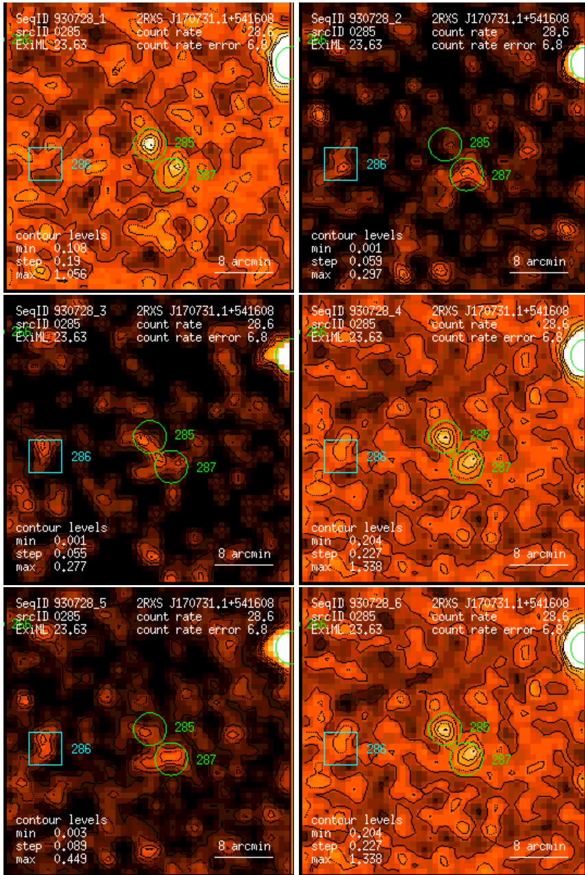
Figure 285: RASS 930728: detection 0285: band rate images, Gaussian filter: (1) PSPC channels 11 – 41, (2) 52 – 90, (3) 91 – 201, (4) 11 – 235, (5) 52 – 201, (6) 11 – 201. Broad band rates in counts/ks. Band rate contour levels in counts/ks/arcmin 2 .
