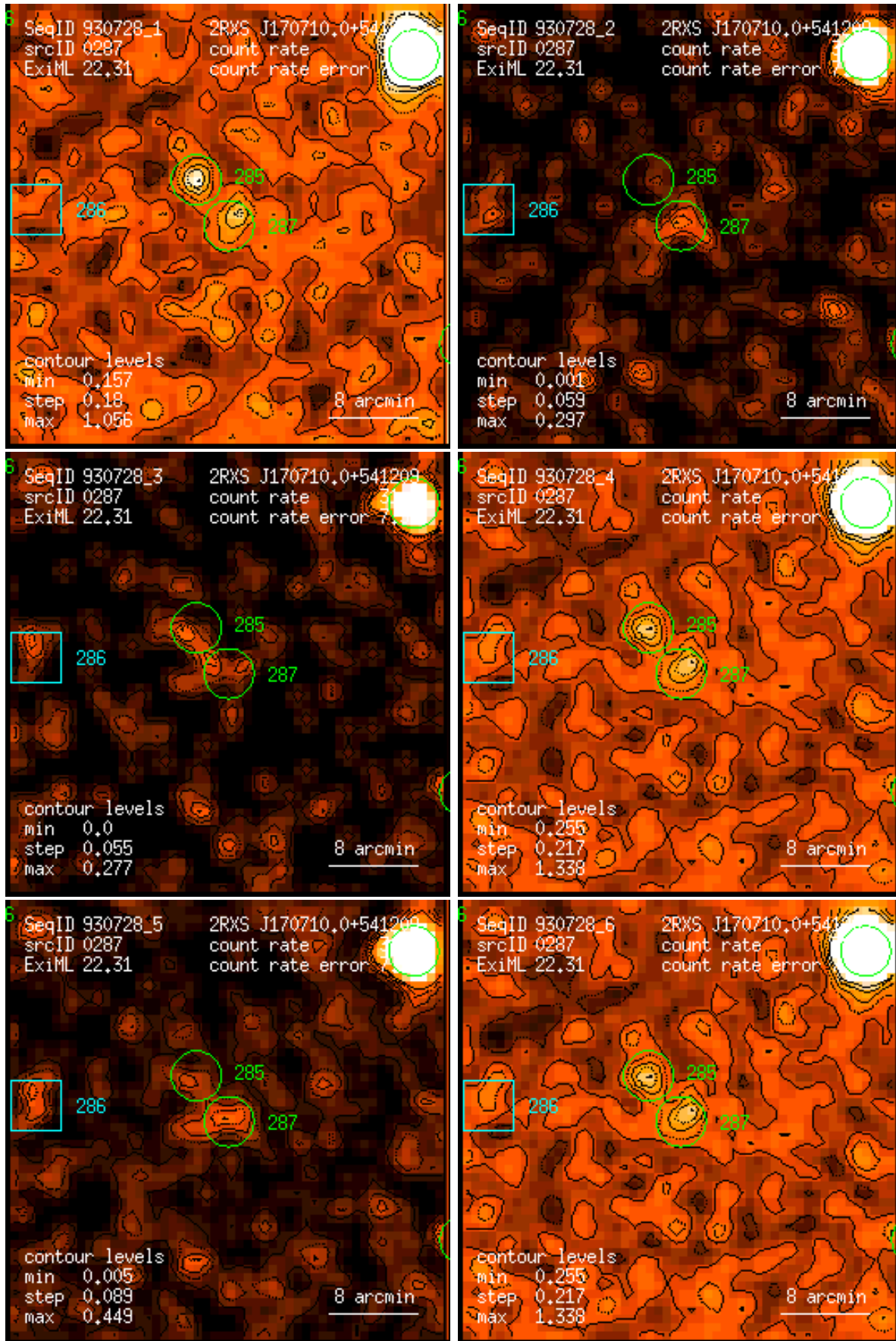
Figure 287: RASS 930728: detection 0287: band rate images, Gaussian filter: (1) PSPC channels 11 – 41, (2) 52 – 90, (3) 91 – 201, (4) 11 – 235, (5) 52 – 201, (6) 11 – 201. Broad band rates in counts/ks. Band rate contour levels in counts/ks/arcmin 2 .
