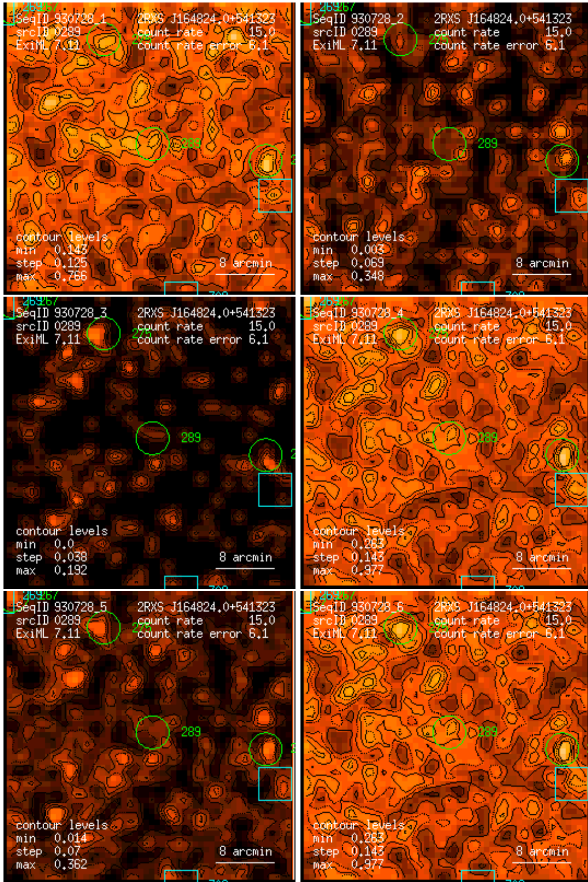
Figure 289: RASS 930728: detection 0289: band rate images, Gaussian filter: (1) PSPC channels 11 – 41, (2) 52 – 90, (3) 91 – 201, (4) 11 – 235, (5) 52 – 201, (6) 11 – 201. Broad band rates in counts/ks. Band rate contour levels in counts/ks/arcmin 2 .
