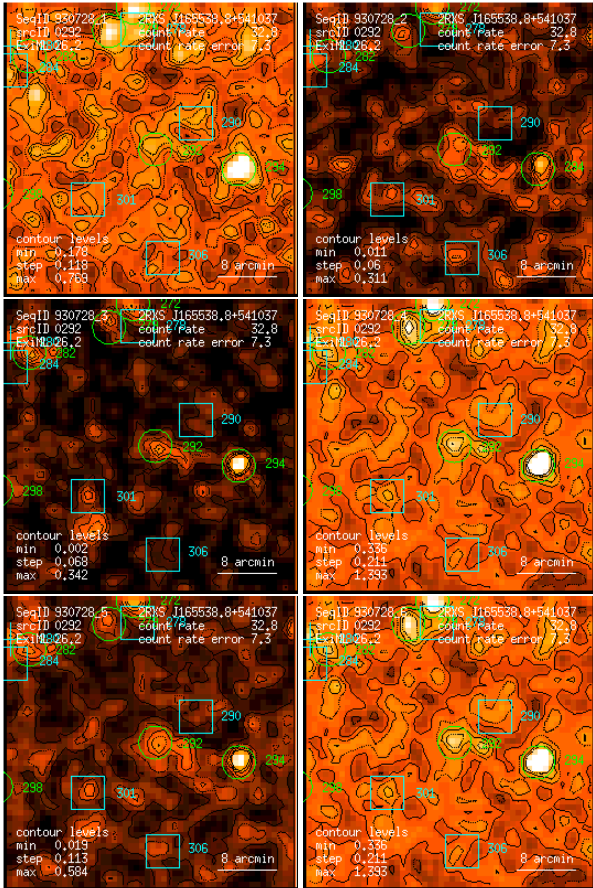
Figure 292: RASS 930728: detection 0292: band rate images, Gaussian filter: (1) PSPC channels 11 – 41, (2) 52 – 90, (3) 91 – 201, (4) 11 – 235, (5) 52 – 201, (6) 11 – 201. Broad band rates in counts/ks. Band rate contour levels in counts/ks/arcmin 2 .
