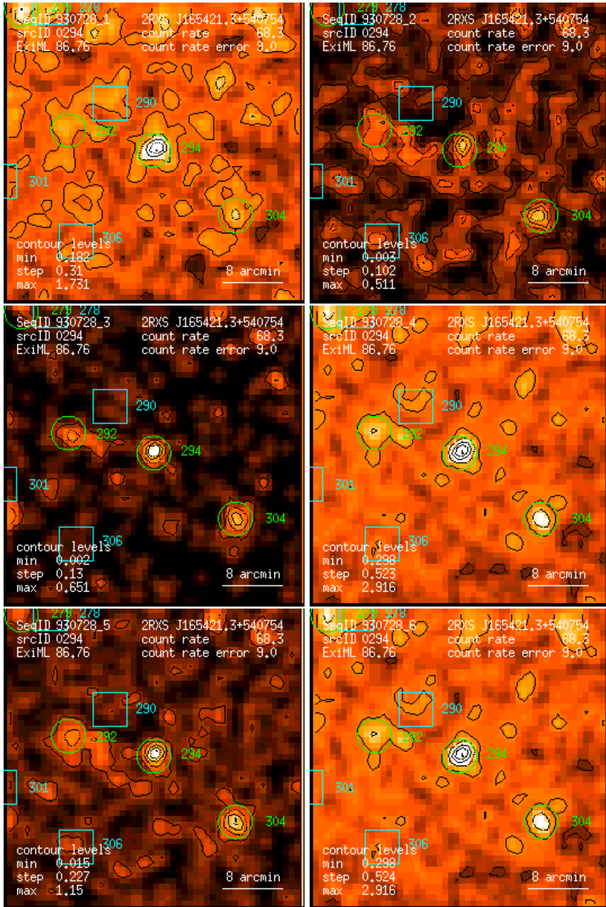
Figure 294: RASS 930728: detection 0294: band rate images, Gaussian filter: (1) PSPC channels 11 – 41, (2) 52 – 90, (3) 91 – 201, (4) 11 – 235, (5) 52 – 201, (6) 11 – 201. Broad band rates in counts/ks. Band rate contour levels in counts/ks/arcmin 2 .
