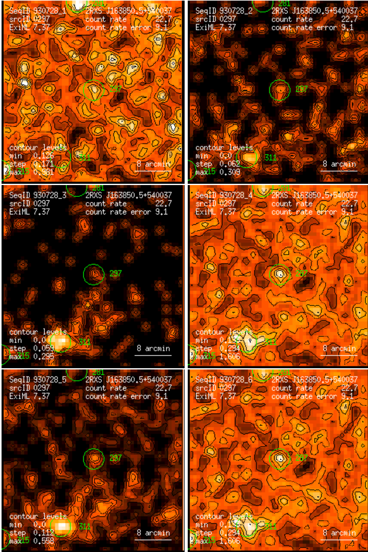
Figure 297: RASS 930728: detection 0297: band rate images, Gaussian filter: (1) PSPC channels 11 – 41, (2) 52 – 90, (3) 91 – 201, (4) 11 – 235, (5) 52 – 201, (6) 11 – 201. Broad band rates in counts/ks. Band rate contour levels in counts/ks/arcmin 2 .
