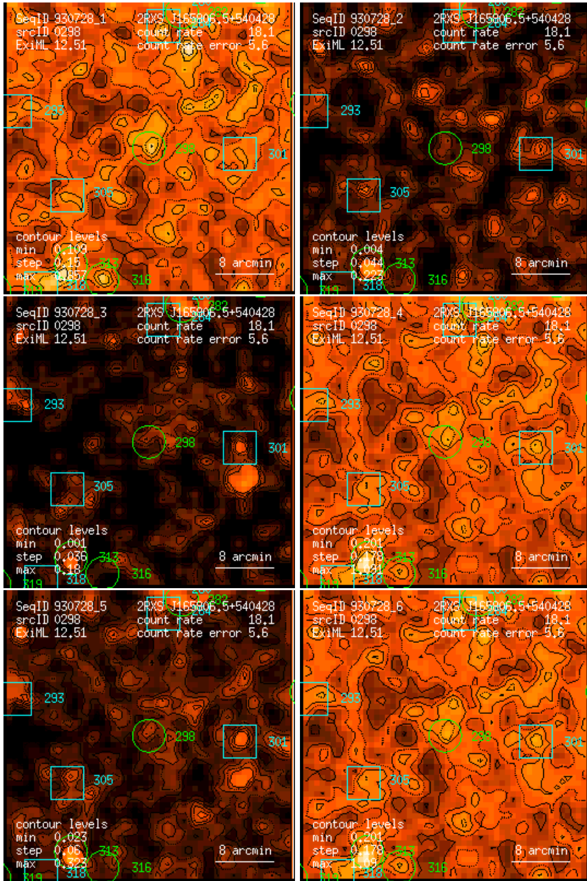
Figure 298: RASS 930728: detection 0298: band rate images, Gaussian filter: (1) PSPC channels 11 – 41, (2) 52 – 90, (3) 91 – 201, (4) 11 – 235, (5) 52 – 201, (6) 11 – 201. Broad band rates in counts/ks. Band rate contour levels in counts/ks/arcmin 2 .
