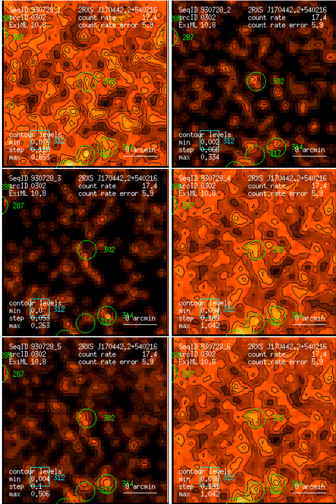
Figure 302: RASS 930728: detection 0302: band rate images, Gaussian filter: (1) PSPC channels 11 – 41, (2) 52 – 90, (3) 91 – 201, (4) 11 – 235, (5) 52 – 201, (6) 11 – 201. Broad band rates in counts/ks. Band rate contour levels in counts/ks/arcmin 2 .
