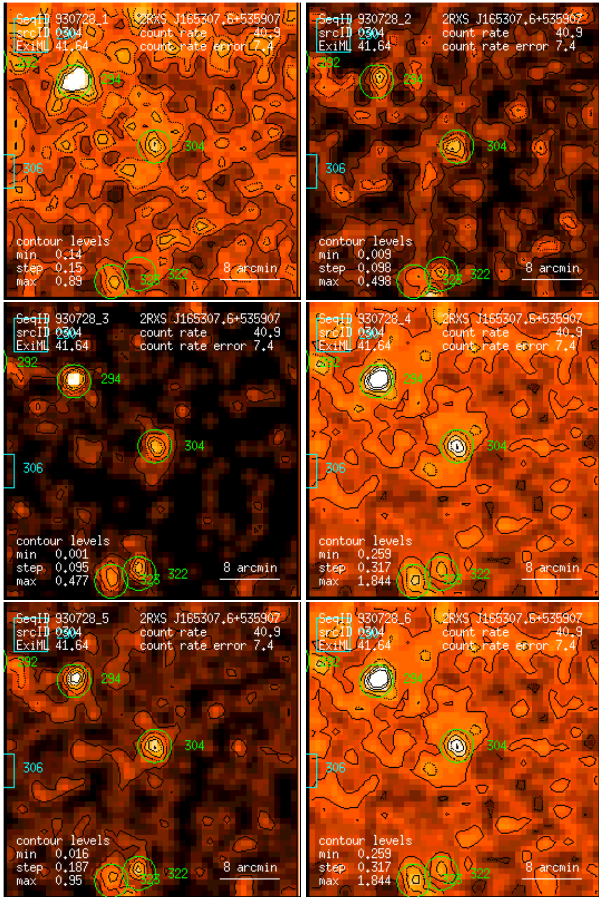
Figure 304: RASS 930728: detection 0304: band rate images, Gaussian filter: (1) PSPC channels 11 – 41, (2) 52 – 90, (3) 91 – 201, (4) 11 – 235, (5) 52 – 201, (6) 11 – 201. Broad band rates in counts/ks. Band rate contour levels in counts/ks/arcmin 2 .
