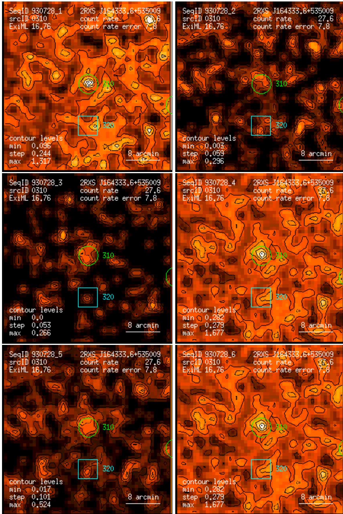
Figure 310: RASS 930728: detection 0310: band rate images, Gaussian filter: (1) PSPC channels 11 – 41, (2) 52 – 90, (3) 91 – 201, (4) 11 – 235, (5) 52 – 201, (6) 11 – 201. Broad band rates in counts/ks. Band rate contour levels in counts/ks/arcmin 2 .
