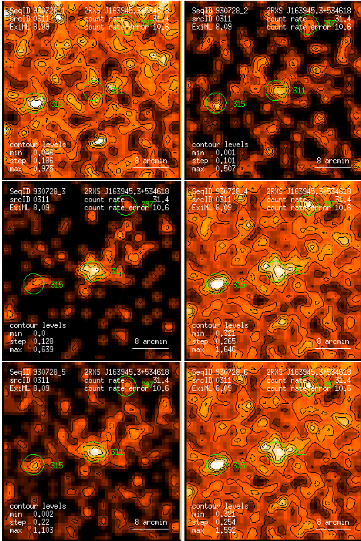
Figure 311: RASS 930728: detection 0311: band rate images, Gaussian filter: (1) PSPC channels 11 – 41, (2) 52 – 90, (3) 91 – 201, (4) 11 – 235, (5) 52 – 201, (6) 11 – 201. Broad band rates in counts/ks. Band rate contour levels in counts/ks/arcmin 2 .
