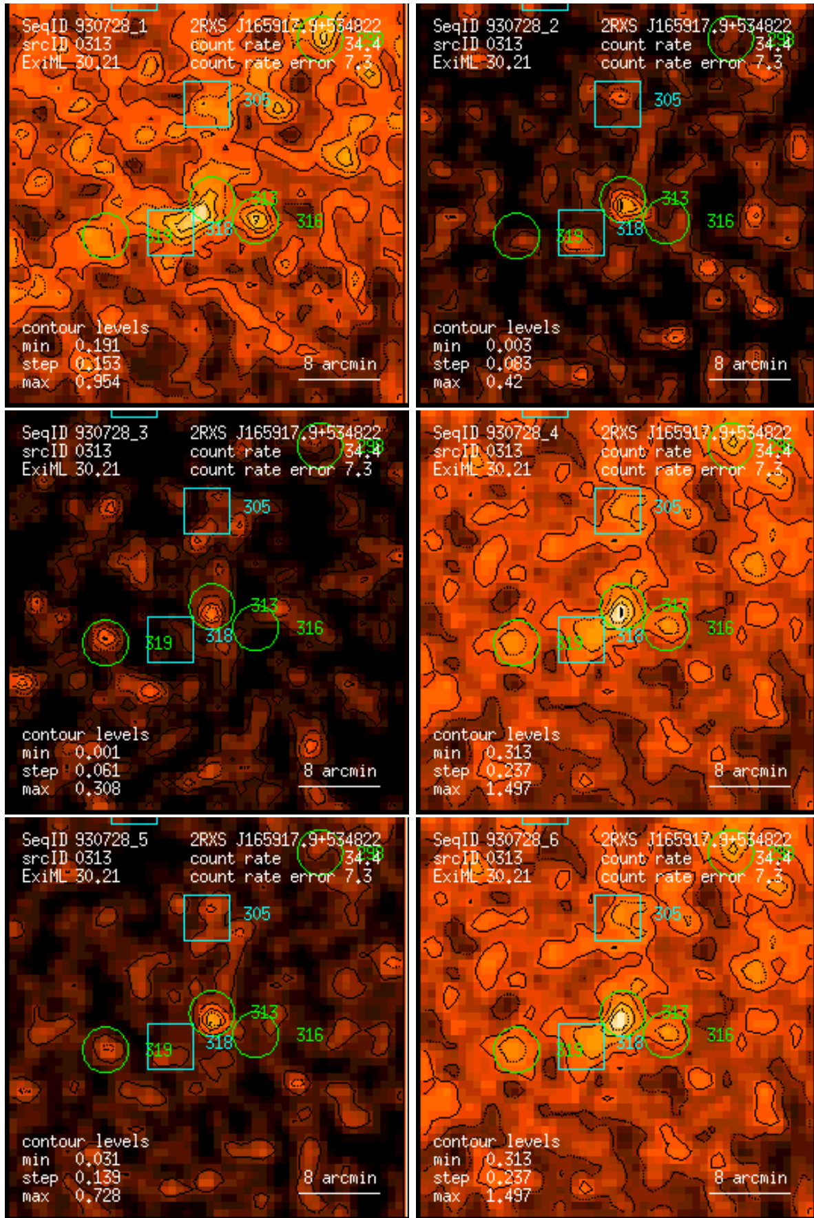
Figure 313: RASS 930728: detection 0313: band rate images, Gaussian filter: (1) PSPC channels 11 – 41, (2) 52 – 90, (3) 91 – 201, (4) 11 – 235, (5) 52 – 201, (6) 11 – 201. Broad band rates in counts/ks. Band rate contour levels in counts/ks/arcmin 2 .
