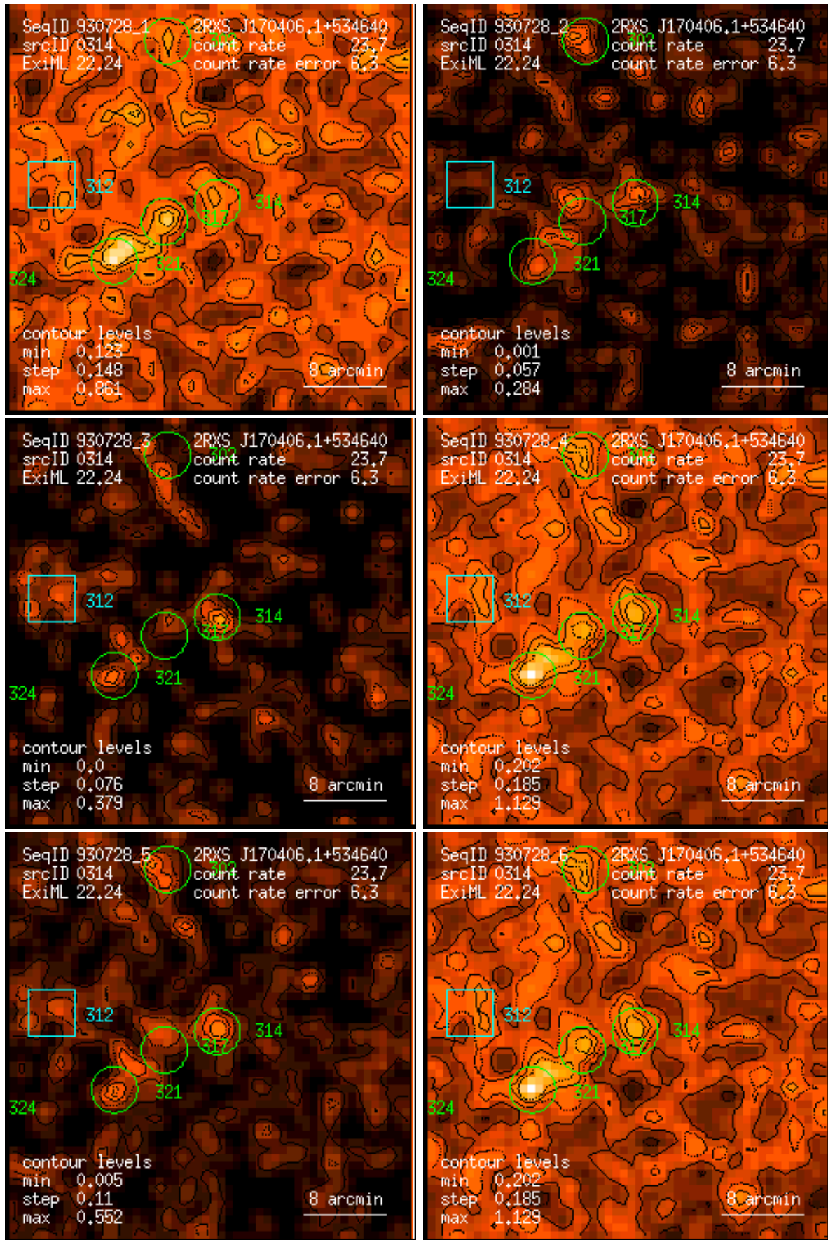
Figure 314: RASS 930728: detection 0314: band rate images, Gaussian filter: (1) PSPC channels 11 – 41, (2) 52 – 90, (3) 91 – 201, (4) 11 – 235, (5) 52 – 201, (6) 11 – 201. Broad band rates in counts/ks. Band rate contour levels in counts/ks/arcmin 2 .
