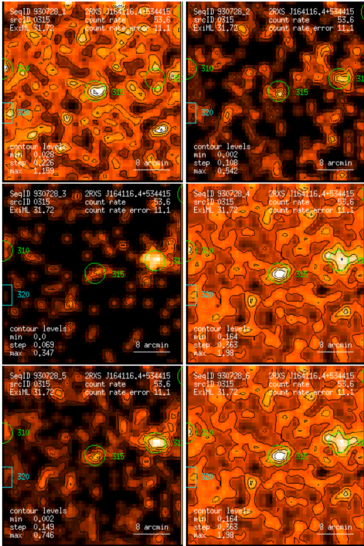
Figure 315: RASS 930728: detection 0315: band rate images, Gaussian filter: (1) PSPC channels 11 – 41, (2) 52 – 90, (3) 91 – 201, (4) 11 – 235, (5) 52 – 201, (6) 11 – 201. Broad band rates in counts/ks. Band rate contour levels in counts/ks/arcmin 2 .
