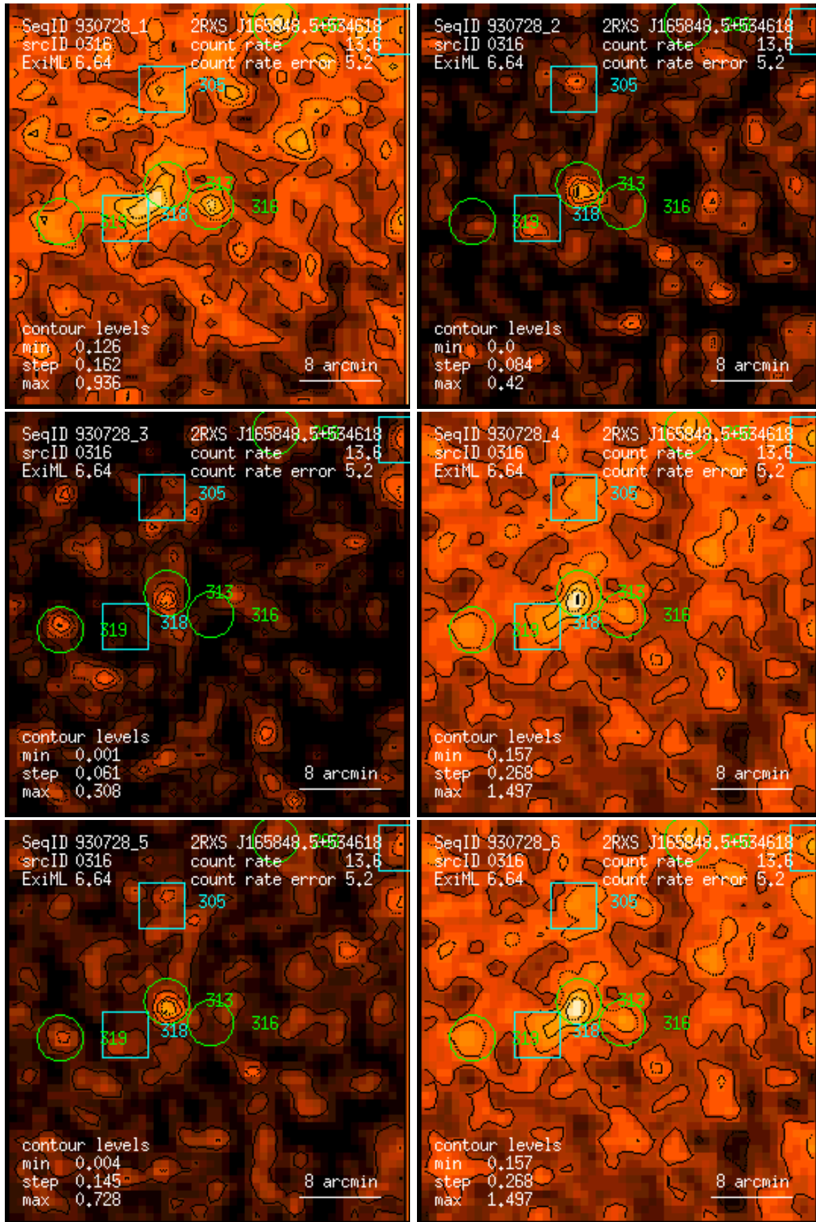
Figure 316: RASS 930728: detection 0316: band rate images, Gaussian filter: (1) PSPC channels 11 – 41, (2) 52 – 90, (3) 91 – 201, (4) 11 – 235, (5) 52 – 201, (6) 11 – 201. Broad band rates in counts/ks. Band rate contour levels in counts/ks/arcmin 2 .
