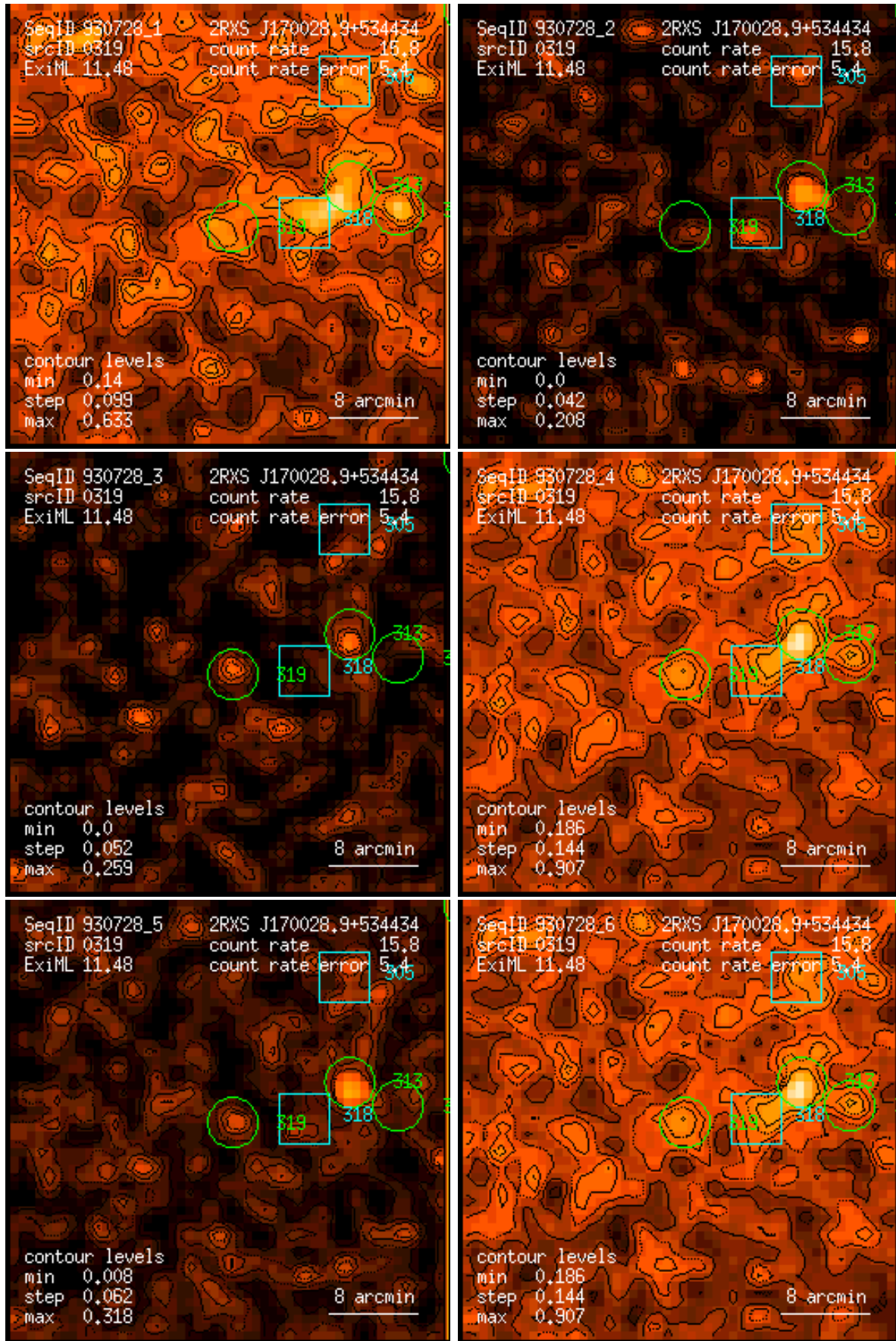
Figure 319: RASS 930728: detection 0319: band rate images, Gaussian filter: (1) PSPC channels 11 – 41, (2) 52 – 90, (3) 91 – 201, (4) 11 – 235, (5) 52 – 201, (6) 11 – 201. Broad band rates in counts/ks. Band rate contour levels in counts/ks/arcmin 2 .
