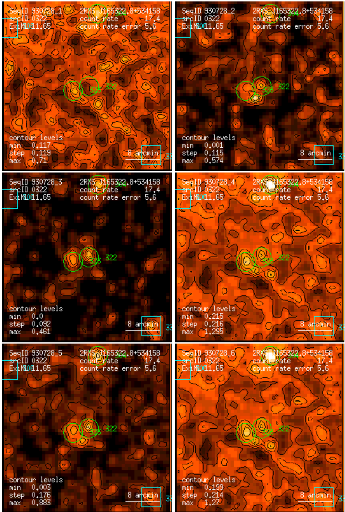
Figure 322: RASS 930728: detection 0322: band rate images, Gaussian filter: (1) PSPC channels 11 – 41, (2) 52 – 90, (3) 91 – 201, (4) 11 – 235, (5) 52 – 201, (6) 11 – 201. Broad band rates in counts/ks. Band rate contour levels in counts/ks/arcmin 2 .
