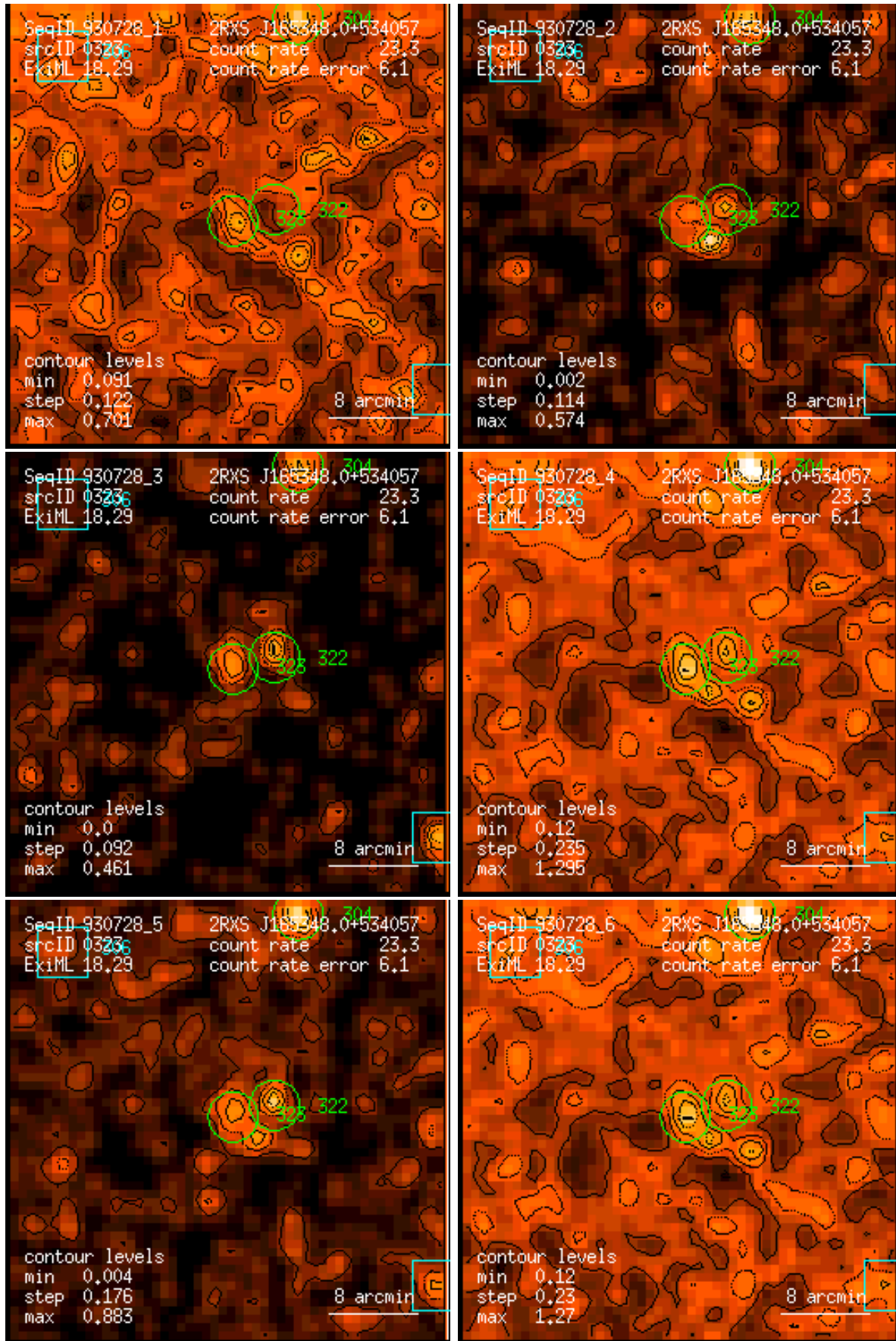
Figure 323: RASS 930728: detection 0323: band rate images, Gaussian filter: (1) PSPC channels 11 – 41, (2) 52 – 90, (3) 91 – 201, (4) 11 – 235, (5) 52 – 201, (6) 11 – 201. Broad band rates in counts/ks. Band rate contour levels in counts/ks/arcmin 2 .
