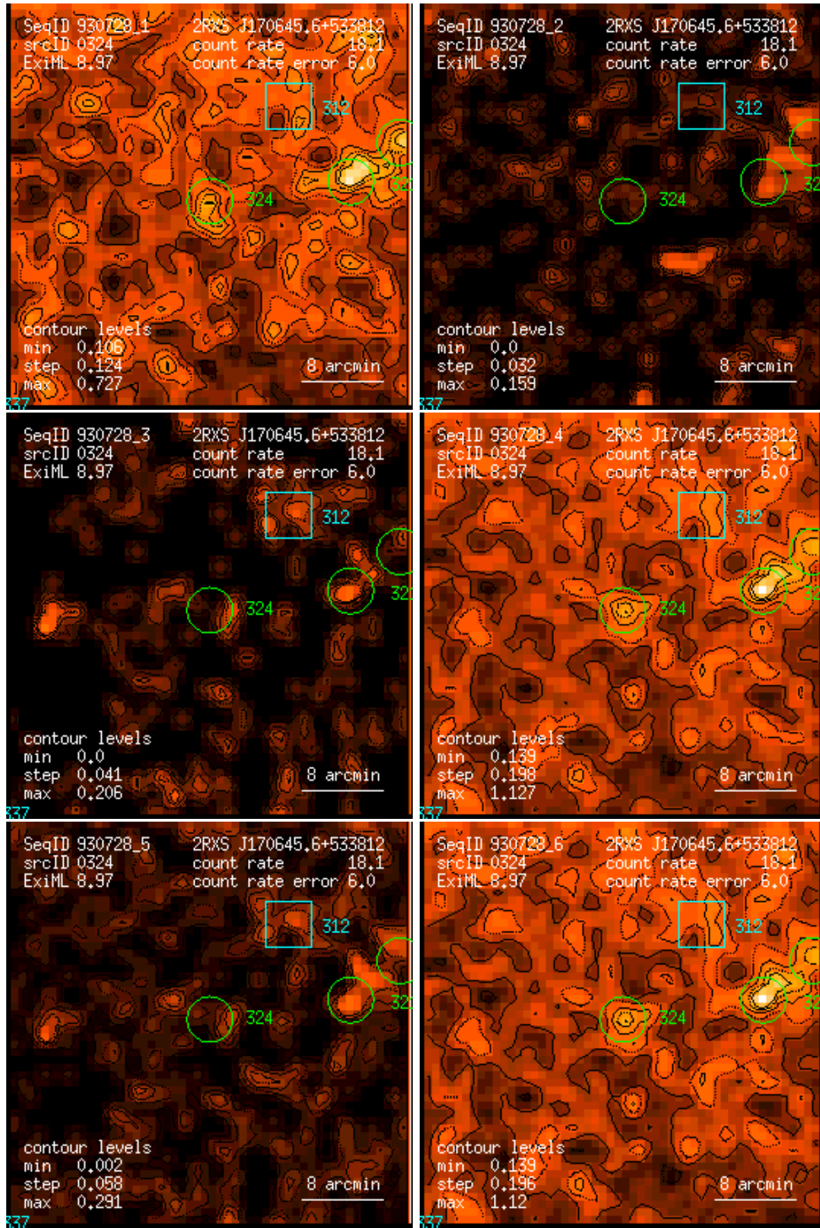
Figure 324: RASS 930728: detection 0324: band rate images, Gaussian filter: (1) PSPC channels 11 – 41, (2) 52 – 90, (3) 91 – 201, (4) 11 – 235, (5) 52 – 201, (6) 11 – 201. Broad band rates in counts/ks. Band rate contour levels in counts/ks/arcmin 2 .
