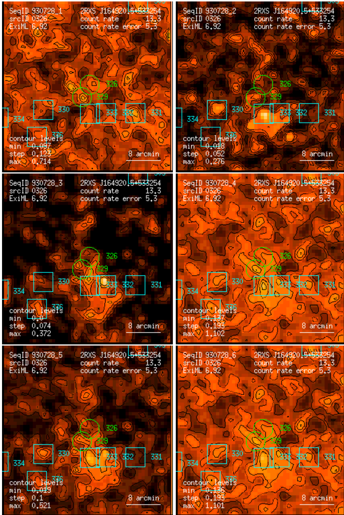
Figure 326: RASS 930728: detection 0326: band rate images, Gaussian filter: (1) PSPC channels 11 – 41, (2) 52 – 90, (3) 91 – 201, (4) 11 – 235, (5) 52 – 201, (6) 11 – 201. Broad band rates in counts/ks. Band rate contour levels in counts/ks/arcmin 2 .
