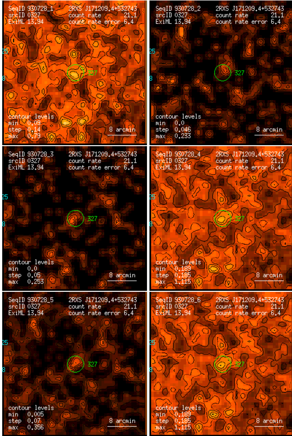
Figure 327: RASS 930728: detection 0327: band rate images, Gaussian filter: (1) PSPC channels 11 – 41, (2) 52 – 90, (3) 91 – 201, (4) 11 – 235, (5) 52 – 201, (6) 11 – 201. Broad band rates in counts/ks. Band rate contour levels in counts/ks/arcmin 2 .
