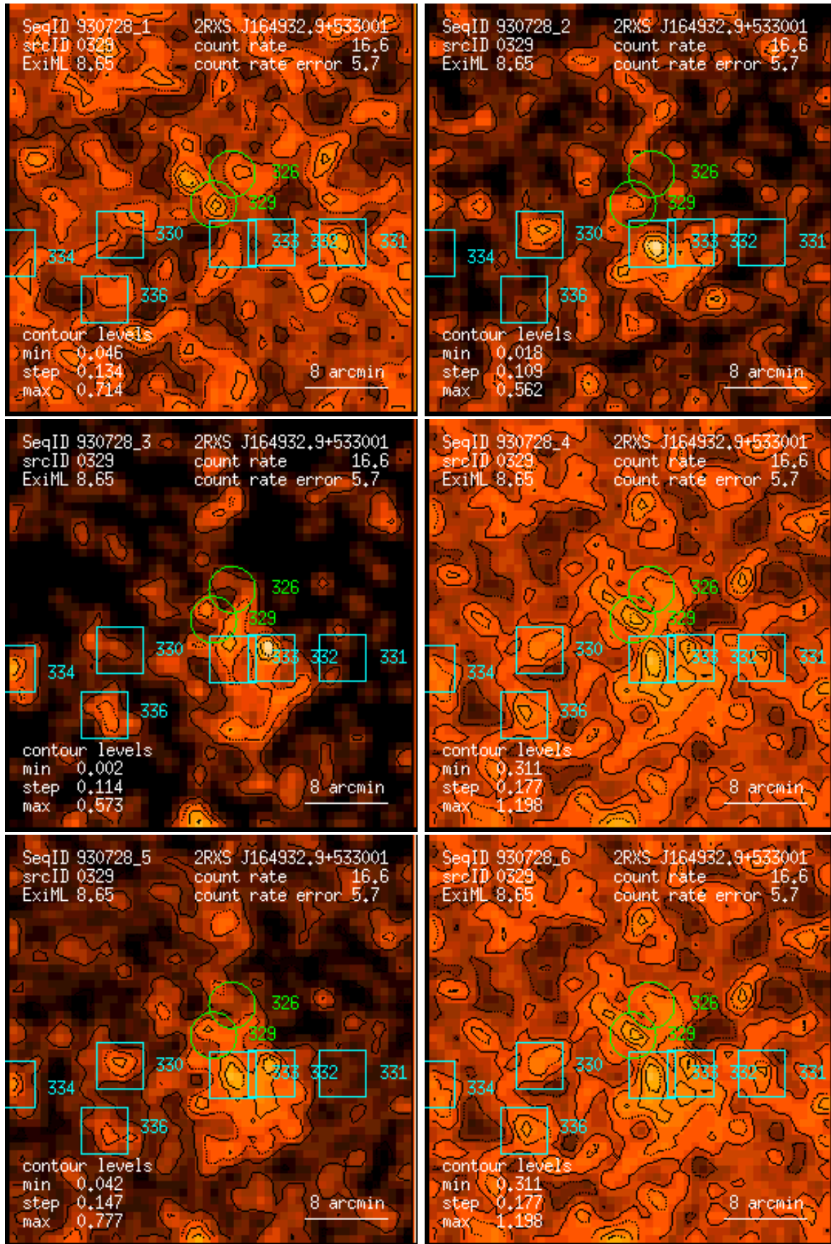
Figure 329: RASS 930728: detection 0329: band rate images, Gaussian filter: (1) PSPC channels 11 – 41, (2) 52 – 90, (3) 91 – 201, (4) 11 – 235, (5) 52 – 201, (6) 11 – 201. Broad band rates in counts/ks. Band rate contour levels in counts/ks/arcmin 2 .
