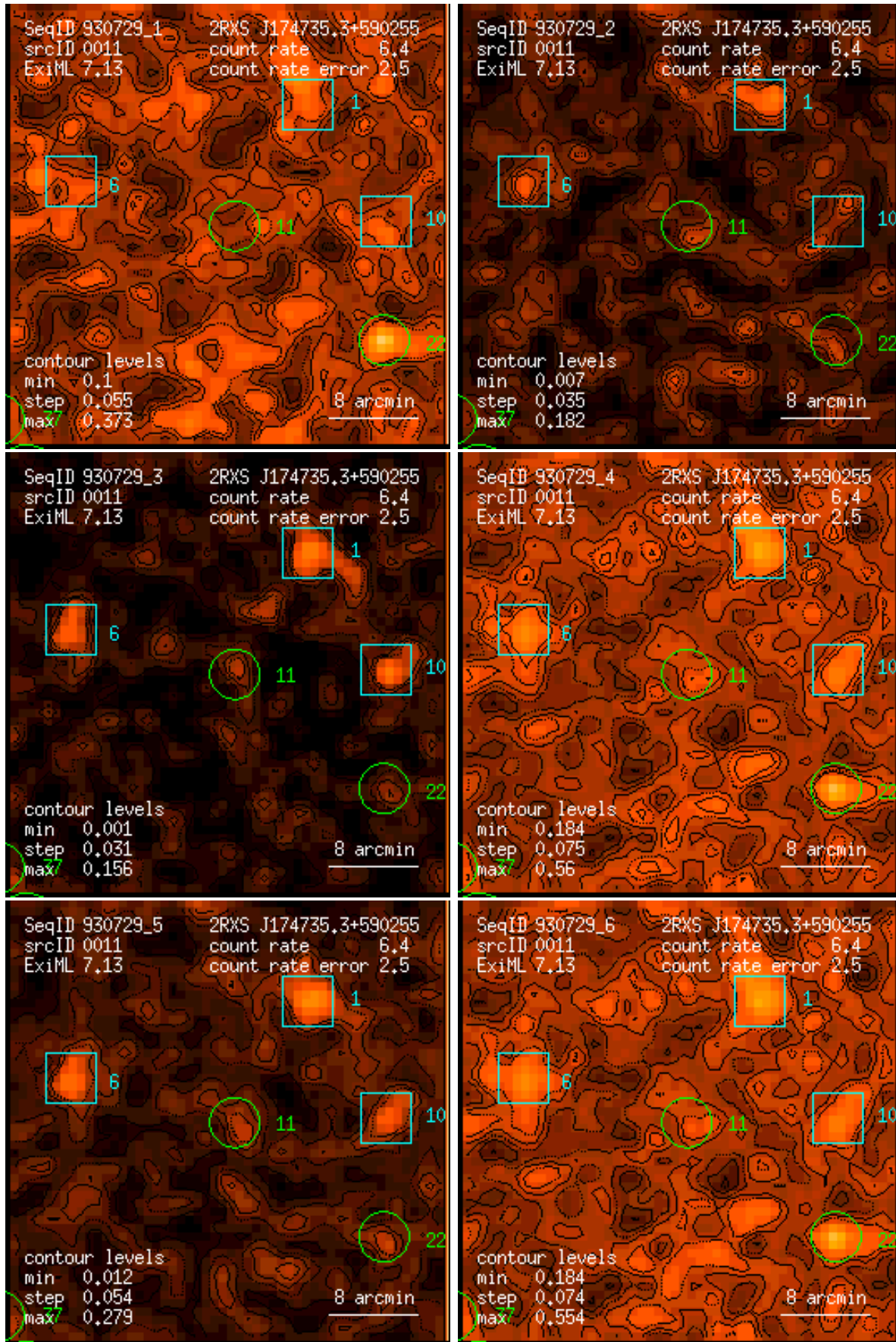
Figure 11: RASS 930729: detection 0011: band rate images, Gaussian filter: (1) PSPC channels 11 – 41, (2) 52 – 90, (3) 91 – 201, (4) 11 – 235, (5) 52 – 201, (6) 11 – 201. Broad band rates in counts/ks. Band rate contour levels in counts/ks/arcmin 2 .
