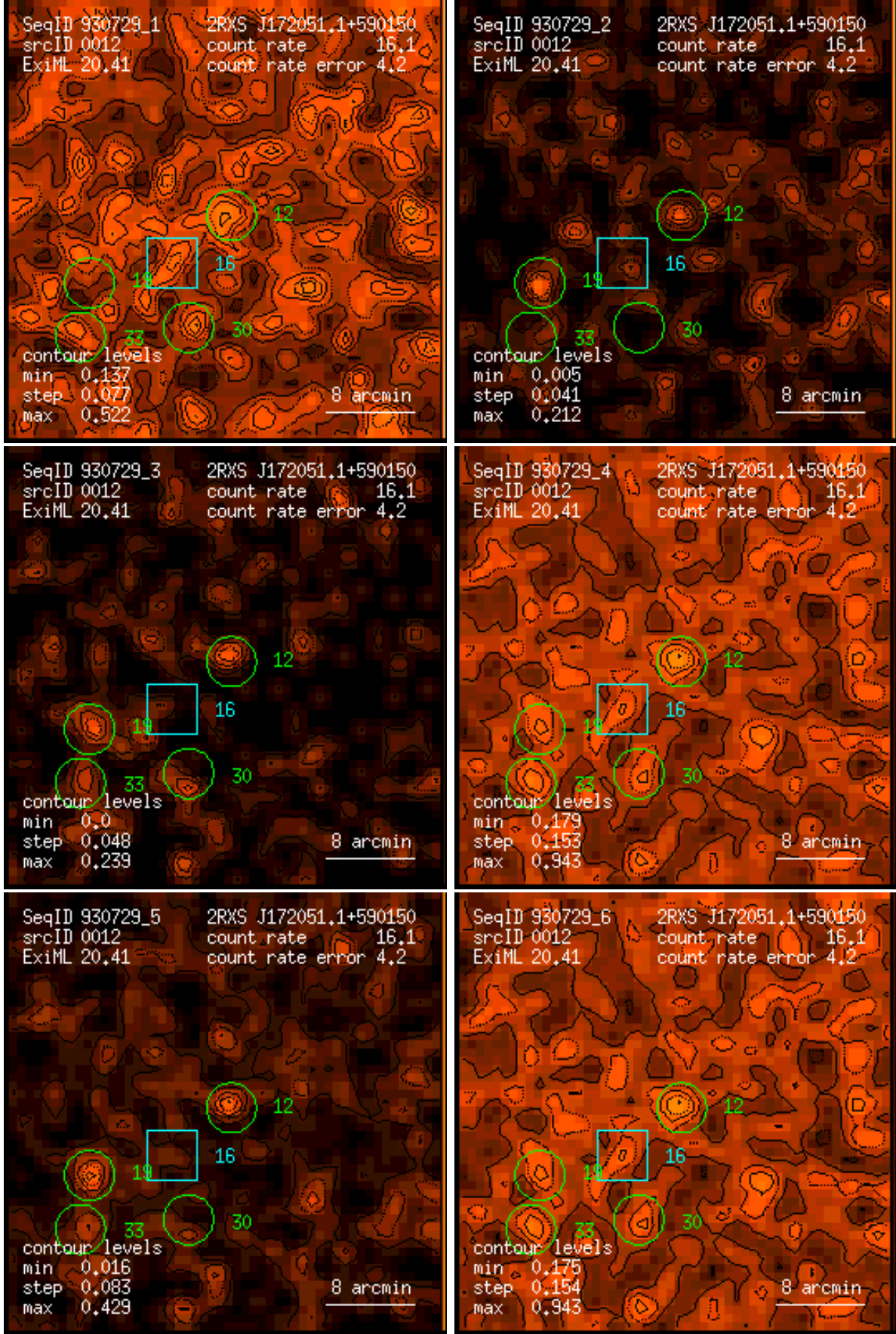
Figure 12: RASS 930729: detection 0012: band rate images, Gaussian filter: (1) PSPC channels 11 – 41, (2) 52 – 90, (3) 91 – 201, (4) 11 – 235, (5) 52 – 201, (6) 11 – 201. Broad band rates in counts/ks. Band rate contour levels in counts/ks/arcmin 2 .
