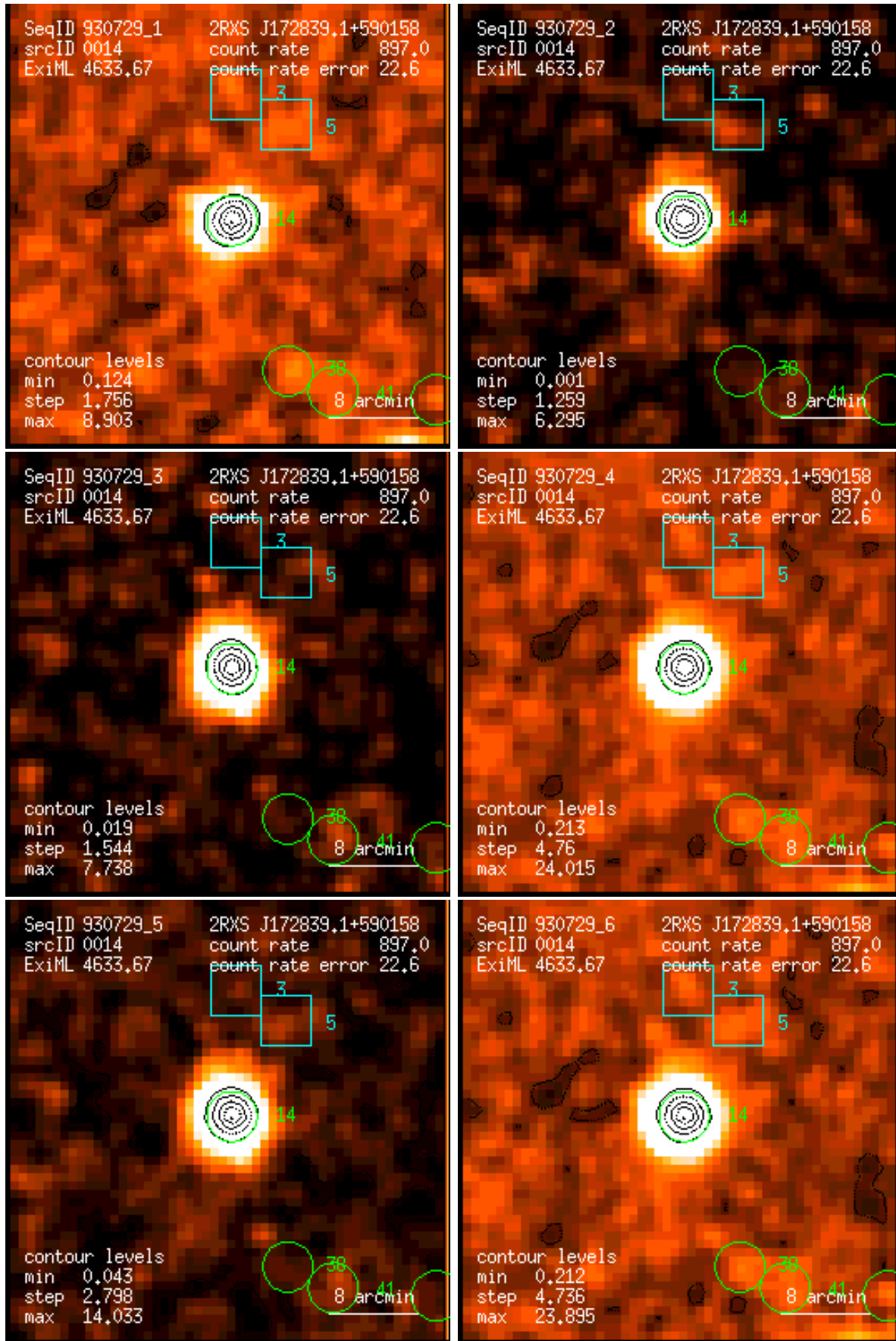
Figure 14: RASS 930729: detection 0014: band rate images, Gaussian filter: (1) PSPC channels 11 – 41, (2) 52 – 90, (3) 91 – 201, (4) 11 – 235, (5) 52 – 201, (6) 11 – 201. Broad band rates in counts/ks. Band rate contour levels in counts/ks/arcmin 2 .
