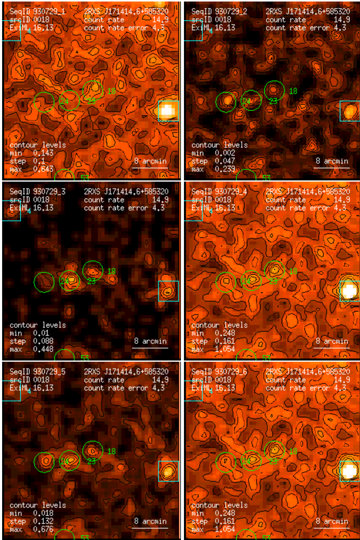
Figure 18: RASS 930729: detection 0018: band rate images, Gaussian filter: (1) PSPC channels 11 – 41, (2) 52 – 90, (3) 91 – 201, (4) 11 – 235, (5) 52 – 201, (6) 11 – 201. Broad band rates in counts/ks. Band rate contour levels in counts/ks/arcmin 2 .
