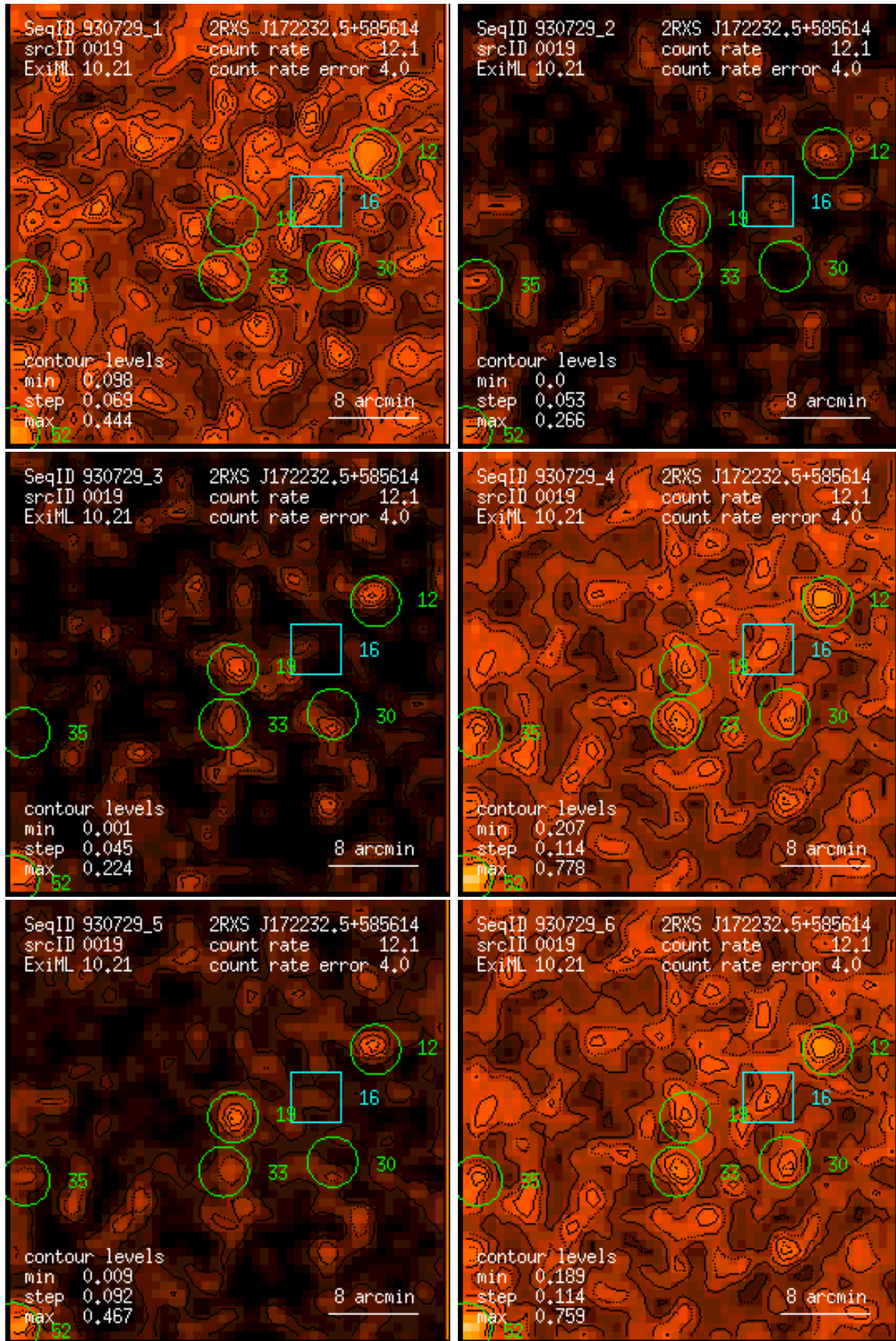
Figure 19: RASS 930729: detection 0019: band rate images, Gaussian filter: (1) PSPC channels 11 – 41, (2) 52 – 90, (3) 91 – 201, (4) 11 – 235, (5) 52 – 201, (6) 11 – 201. Broad band rates in counts/ks. Band rate contour levels in counts/ks/arcmin 2 .
