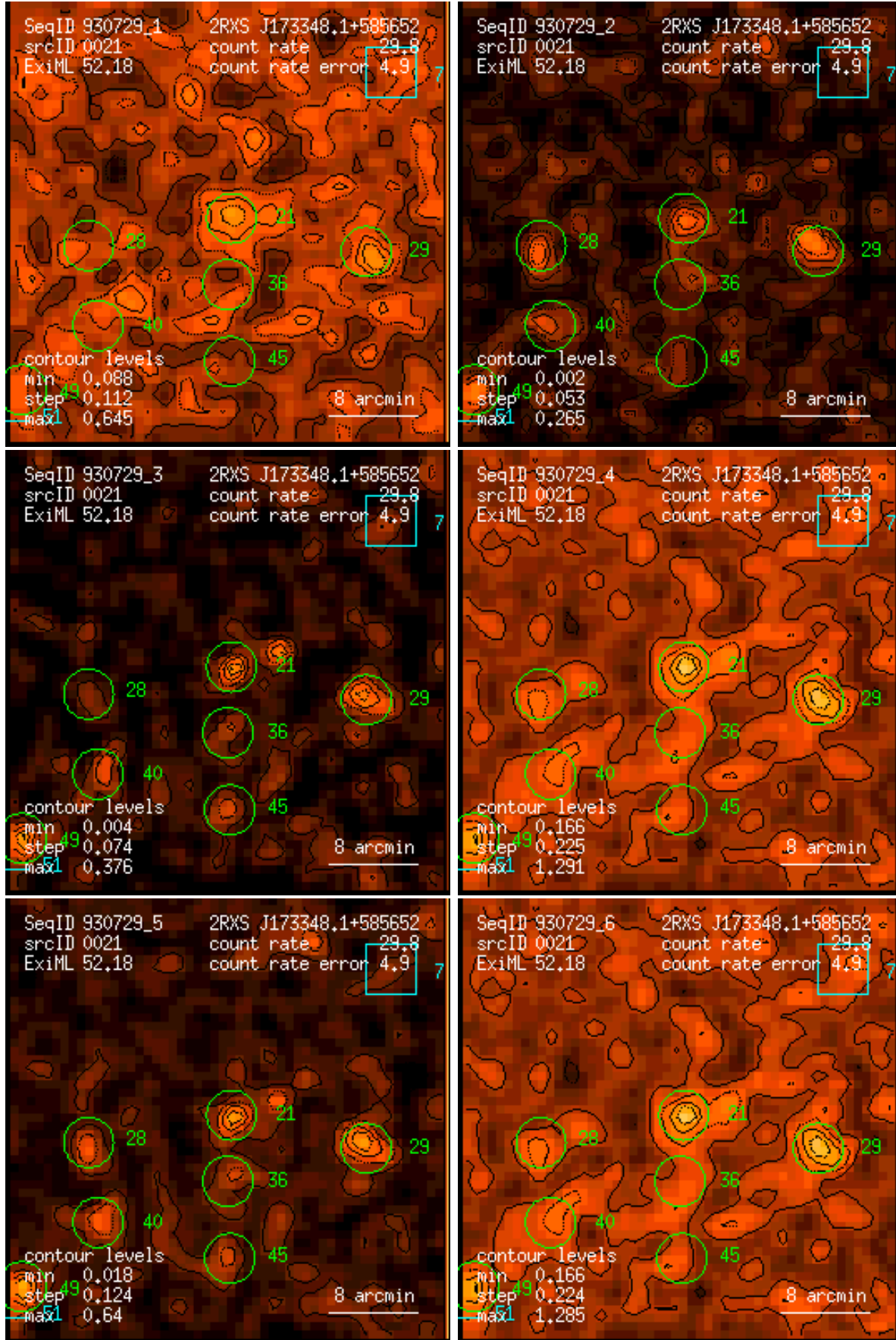
Figure 21: RASS 930729: detection 0021: band rate images, Gaussian filter: (1) PSPC channels 11 – 41, (2) 52 – 90, (3) 91 – 201, (4) 11 – 235, (5) 52 – 201, (6) 11 – 201. Broad band rates in counts/ks. Band rate contour levels in counts/ks/arcmin 2 .
